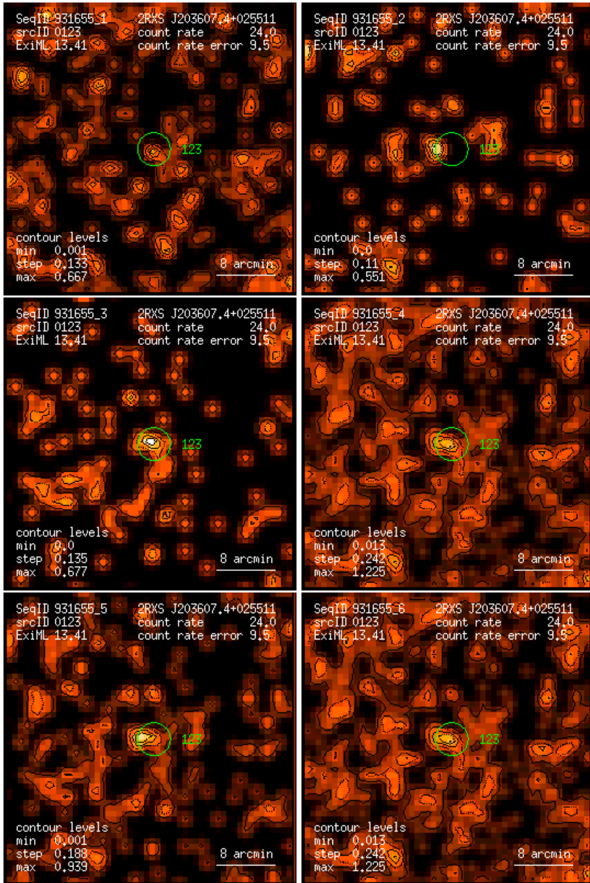
Figure 123: RASS 931655: detection 0123: band rate images, Gaussian filter: (1) PSPC channels 11 – 41, (2) 52 – 90, (3) 91 – 201, (4) 11 – 235, (5) 52 – 201, (6) 11 – 201. Broad band rates in counts/ks. Band rate contour levels in counts/ks/arcmin 2 .
