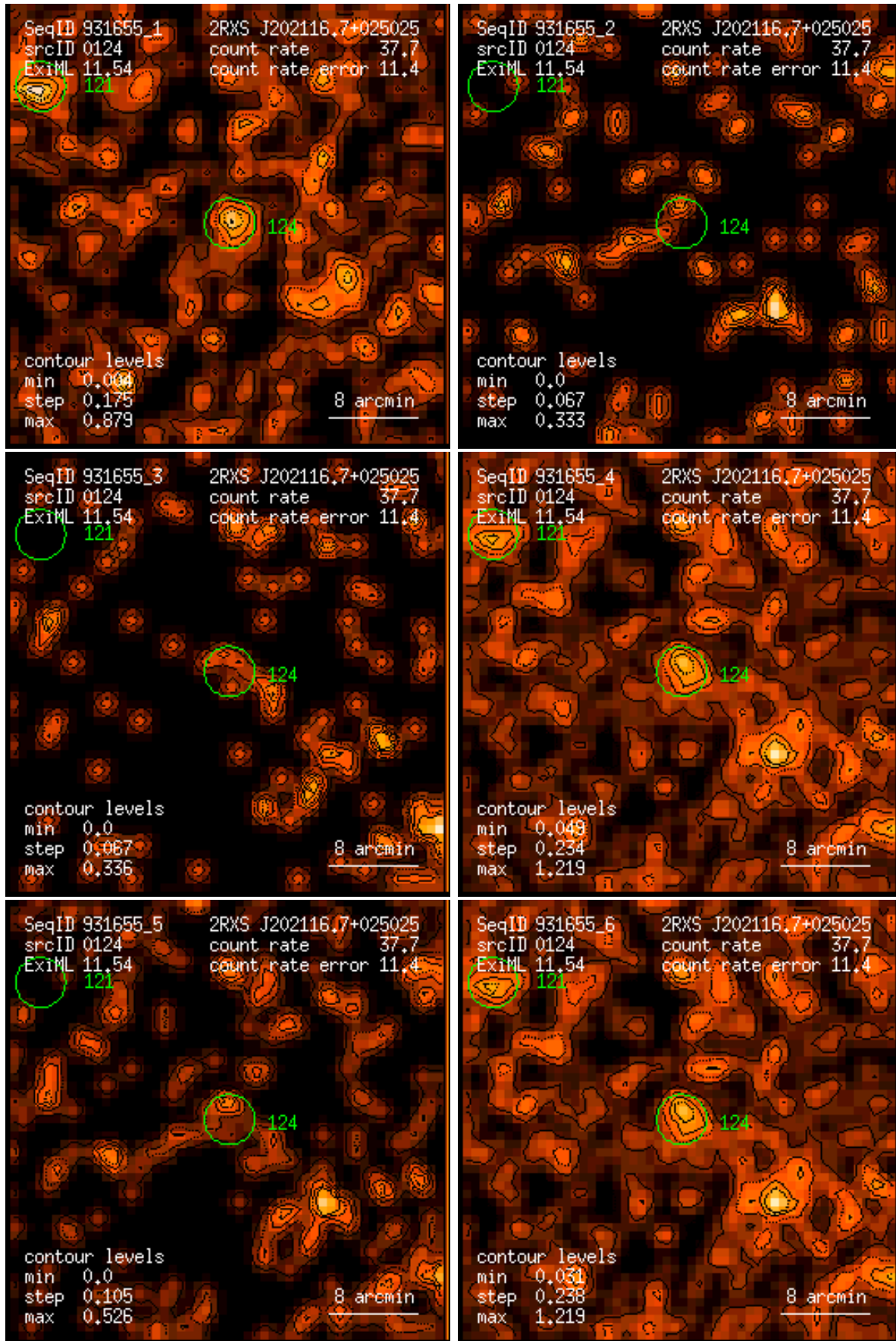
Figure 124: RASS 931655: detection 0124: band rate images, Gaussian filter: (1) PSPC channels 11 – 41, (2) 52 – 90, (3) 91 – 201, (4) 11 – 235, (5) 52 – 201, (6) 11 – 201. Broad band rates in counts/ks. Band rate contour levels in counts/ks/arcmin 2 .
