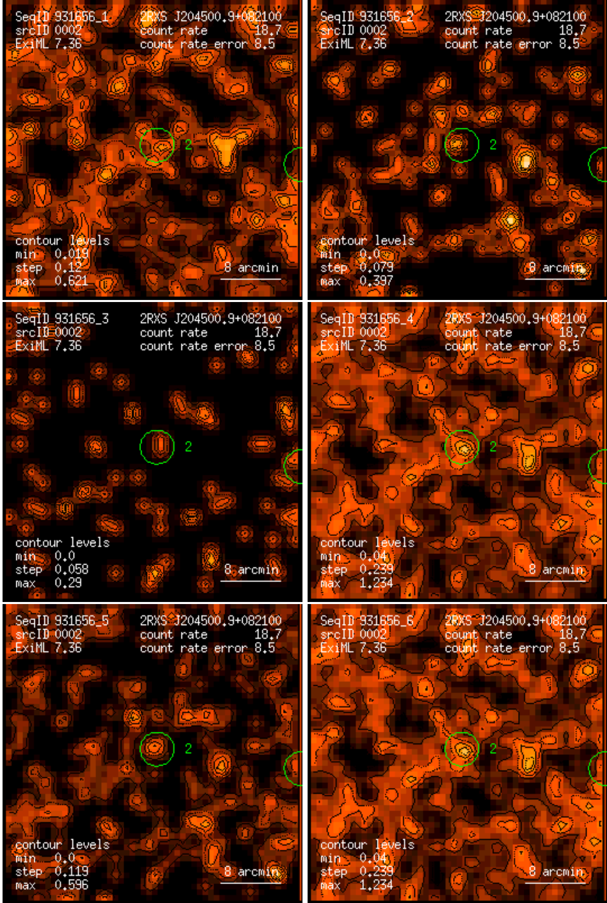
Figure 2: RASS 931656: detection 0002: band rate images, Gaussian filter: (1) PSPC channels 11 – 41, (2) 52 – 90, (3) 91 – 201, (4) 11 – 235, (5) 52 – 201, (6) 11 – 201. Broad band rates in counts/ks. Band rate contour levels in counts/ks/arcmin 2 .
