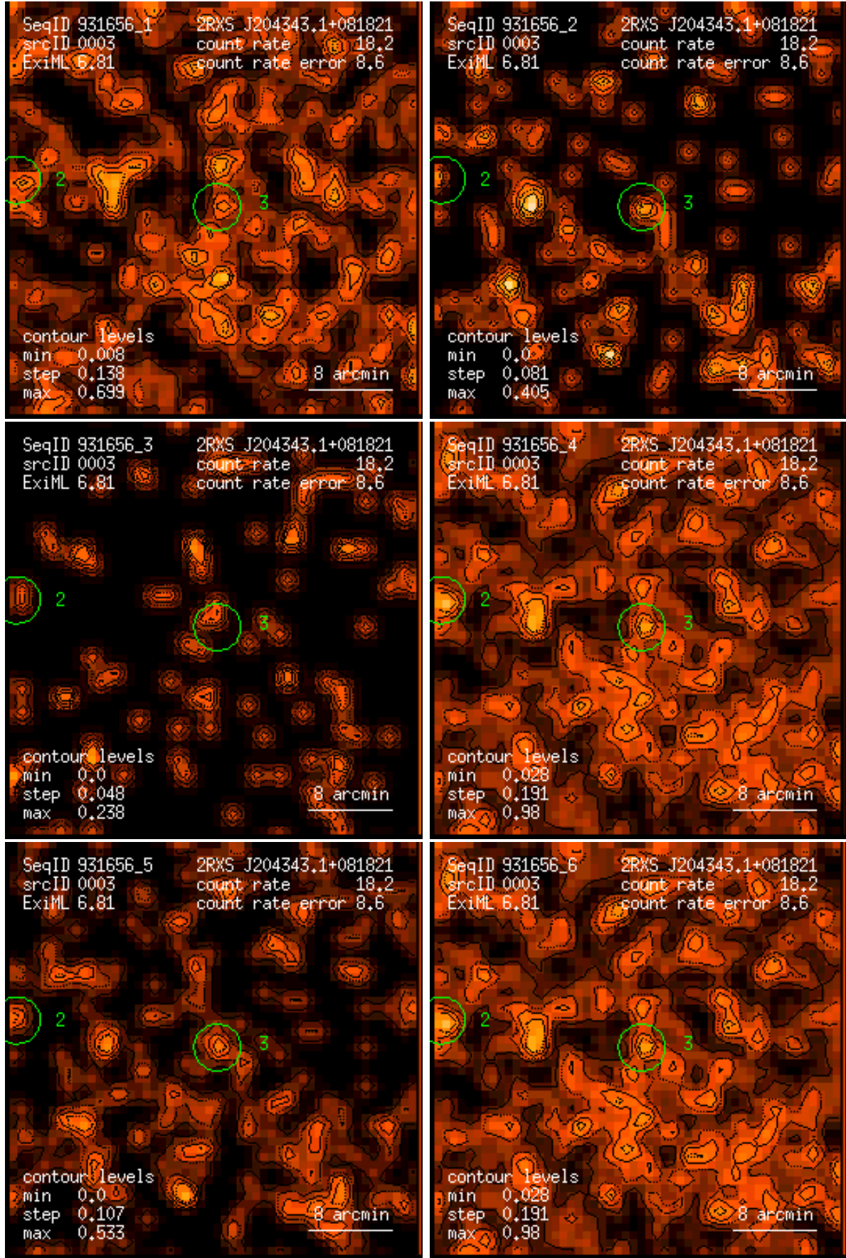
Figure 3: RASS 931656: detection 0003: band rate images, Gaussian filter: (1) PSPC channels 11 – 41, (2) 52 – 90, (3) 91 – 201, (4) 11 – 235, (5) 52 – 201, (6) 11 – 201. Broad band rates in counts/ks. Band rate contour levels in counts/ks/arcmin 2 .
