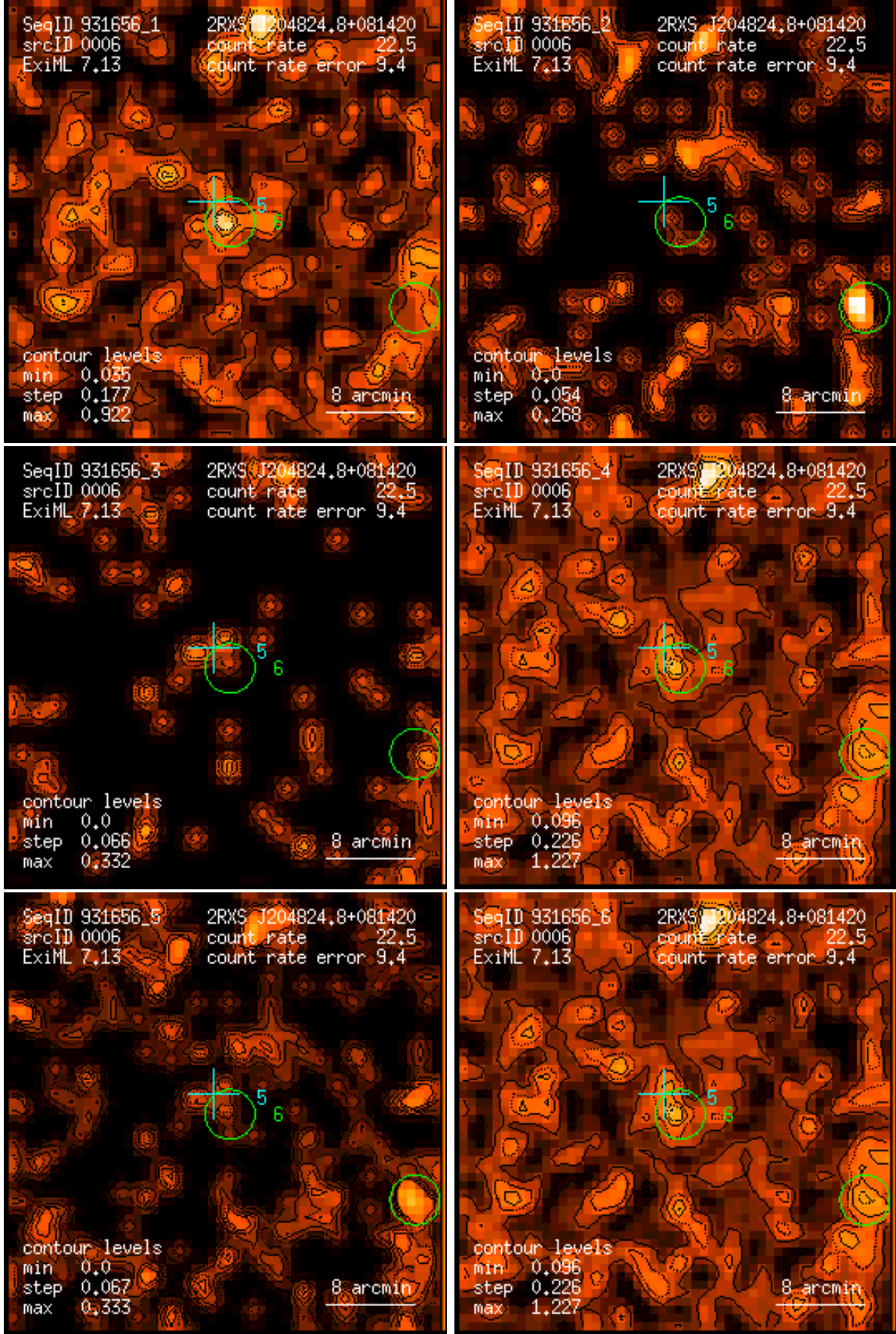
Figure 6: RASS 931656: detection 0006: band rate images, Gaussian filter: (1) PSPC channels 11 – 41, (2) 52 – 90, (3) 91 – 201, (4) 11 – 235, (5) 52 – 201, (6) 11 – 201. Broad band rates in counts/ks. Band rate contour levels in counts/ks/arcmin 2 .
