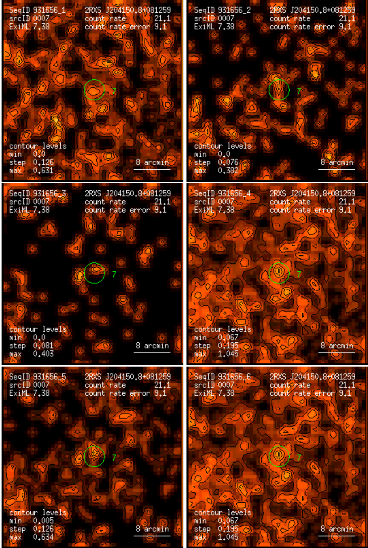
Figure 7: RASS 931656: detection 0007: band rate images, Gaussian filter: (1) PSPC channels 11 – 41, (2) 52 – 90, (3) 91 – 201, (4) 11 – 235, (5) 52 – 201, (6) 11 – 201. Broad band rates in counts/ks. Band rate contour levels in counts/ks/arcmin 2 .
