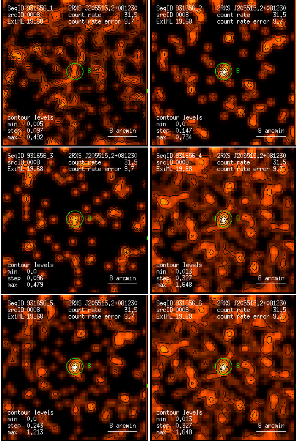
Figure 8: RASS 931656: detection 0008: band rate images, Gaussian filter: (1) PSPC channels 11 – 41, (2) 52 – 90, (3) 91 – 201, (4) 11 – 235, (5) 52 – 201, (6) 11 – 201. Broad band rates in counts/ks. Band rate contour levels in counts/ks/arcmin 2 .
