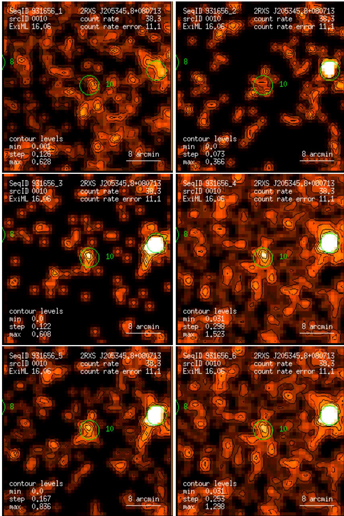
Figure 10: RASS 931656: detection 0010: band rate images, Gaussian filter: (1) PSPC channels 11 – 41, (2) 52 – 90, (3) 91 – 201, (4) 11 – 235, (5) 52 – 201, (6) 11 – 201. Broad band rates in counts/ks. Band rate contour levels in counts/ks/arcmin 2 .
