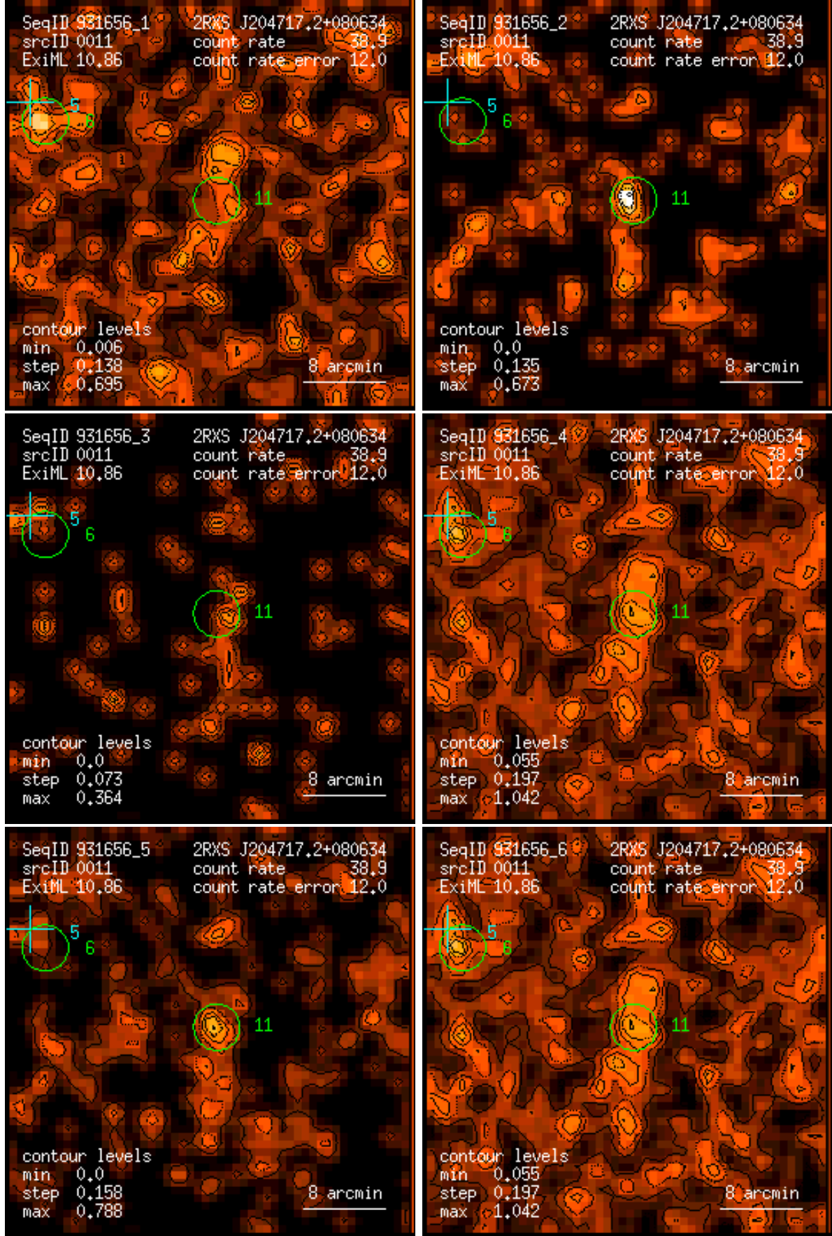
Figure 11: RASS 931656: detection 0011: band rate images, Gaussian filter: (1) PSPC channels 11 – 41, (2) 52 – 90, (3) 91 – 201, (4) 11 – 235, (5) 52 – 201, (6) 11 – 201. Broad band rates in counts/ks. Band rate contour levels in counts/ks/arcmin 2 .
