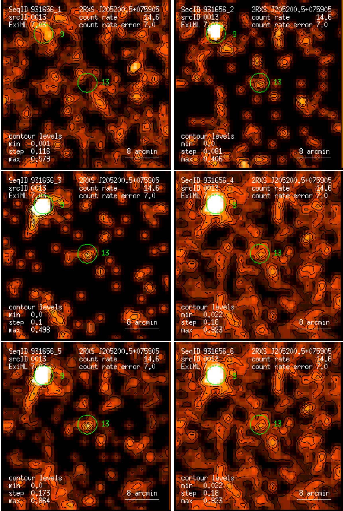
Figure 13: RASS 931656: detection 0013: band rate images, Gaussian filter: (1) PSPC channels 11 – 41, (2) 52 – 90, (3) 91 – 201, (4) 11 – 235, (5) 52 – 201, (6) 11 – 201. Broad band rates in counts/ks. Band rate contour levels in counts/ks/arcmin 2 .
