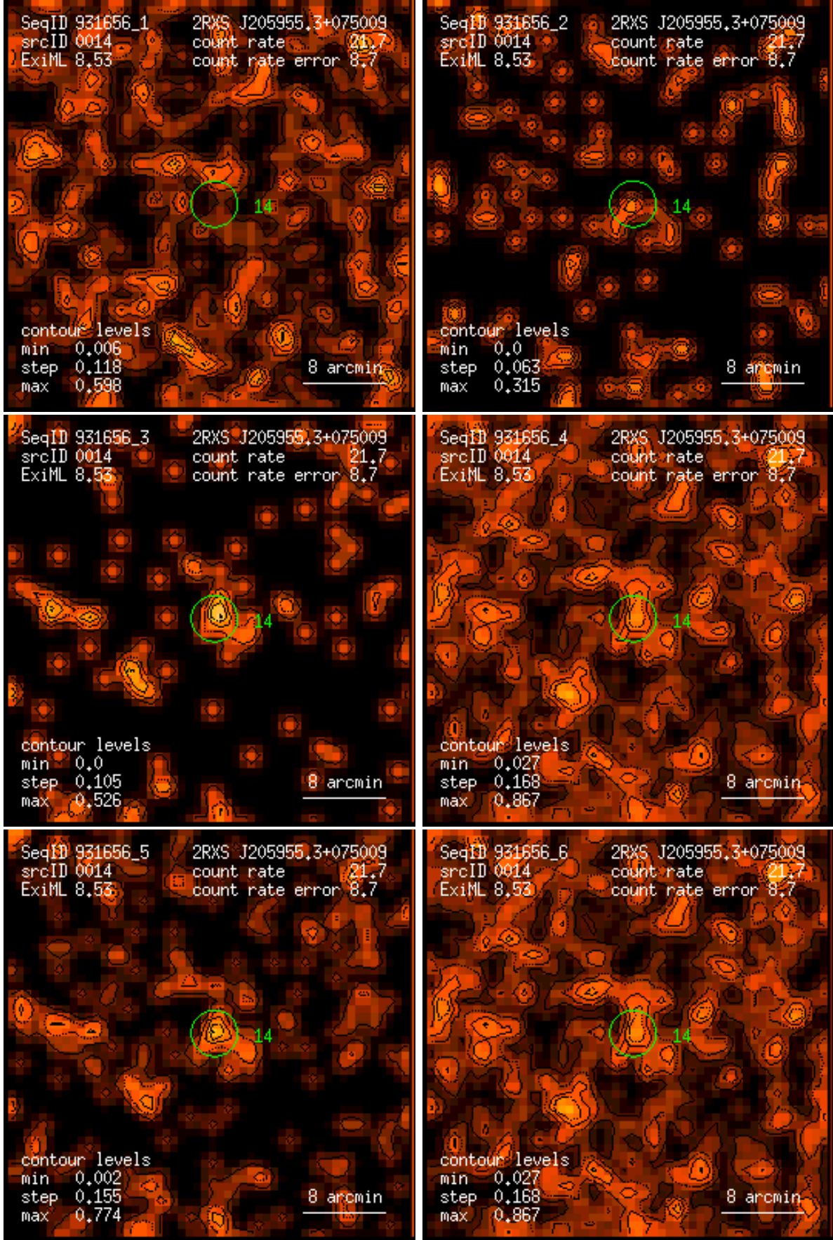
Figure 14: RASS 931656: detection 0014: band rate images, Gaussian filter: (1) PSPC channels 11 – 41, (2) 52 – 90, (3) 91 – 201, (4) 11 – 235, (5) 52 – 201, (6) 11 – 201. Broad band rates in counts/ks. Band rate contour levels in counts/ks/arcmin 2 .
