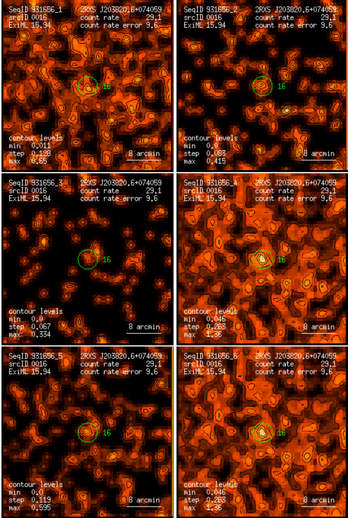
Figure 16: RASS 931656: detection 0016: band rate images, Gaussian filter: (1) PSPC channels 11 – 41, (2) 52 – 90, (3) 91 – 201, (4) 11 – 235, (5) 52 – 201, (6) 11 – 201. Broad band rates in counts/ks. Band rate contour levels in counts/ks/arcmin 2 .
