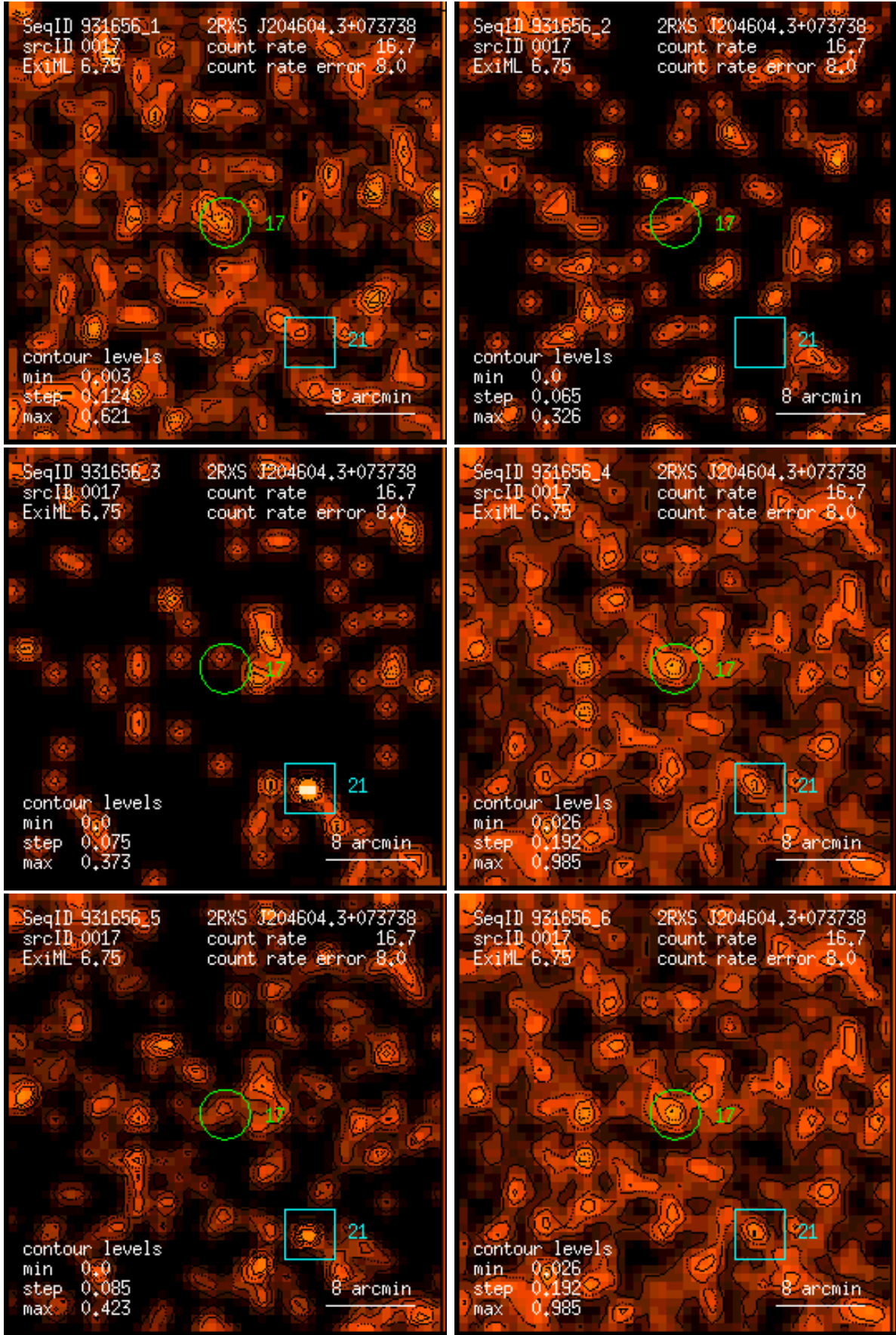
Figure 17: RASS 931656: detection 0017: band rate images, Gaussian filter: (1) PSPC channels 11 – 41, (2) 52 – 90, (3) 91 – 201, (4) 11 – 235, (5) 52 – 201, (6) 11 – 201. Broad band rates in counts/ks. Band rate contour levels in counts/ks/arcmin 2 .
