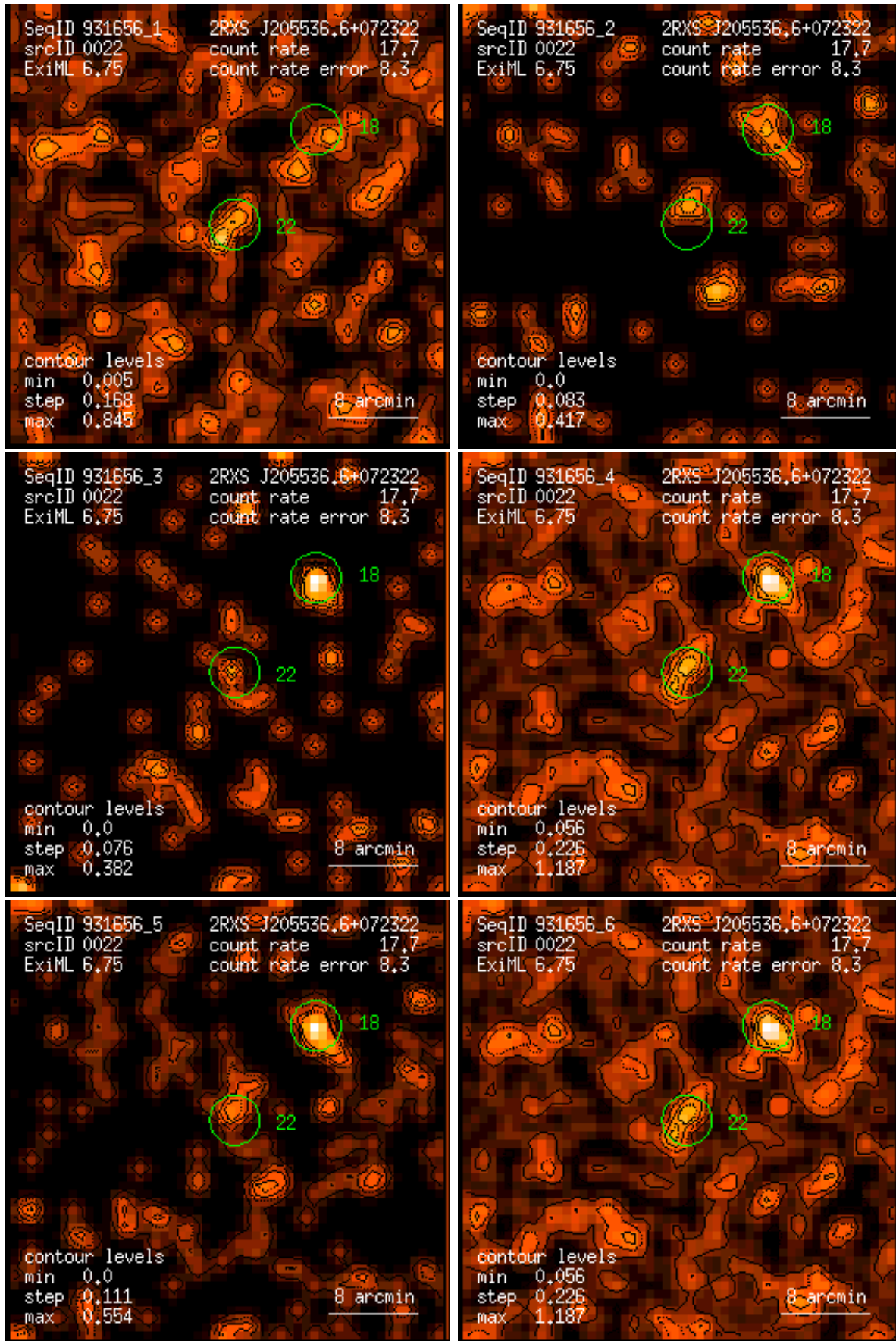
Figure 22: RASS 931656: detection 0022: band rate images, Gaussian filter: (1) PSPC channels 11 – 41, (2) 52 – 90, (3) 91 – 201, (4) 11 – 235, (5) 52 – 201, (6) 11 – 201. Broad band rates in counts/ks. Band rate contour levels in counts/ks/arcmin 2 .
