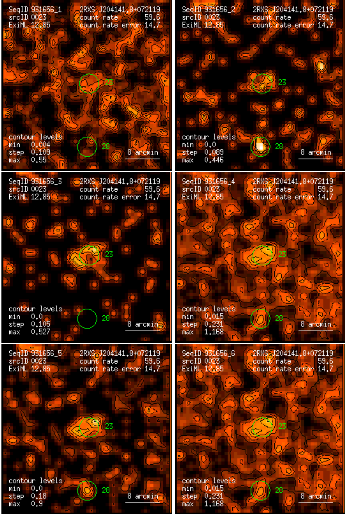
Figure 23: RASS 931656: detection 0023: band rate images, Gaussian filter: (1) PSPC channels 11 – 41, (2) 52 – 90, (3) 91 – 201, (4) 11 – 235, (5) 52 – 201, (6) 11 – 201. Broad band rates in counts/ks. Band rate contour levels in counts/ks/arcmin 2 .
