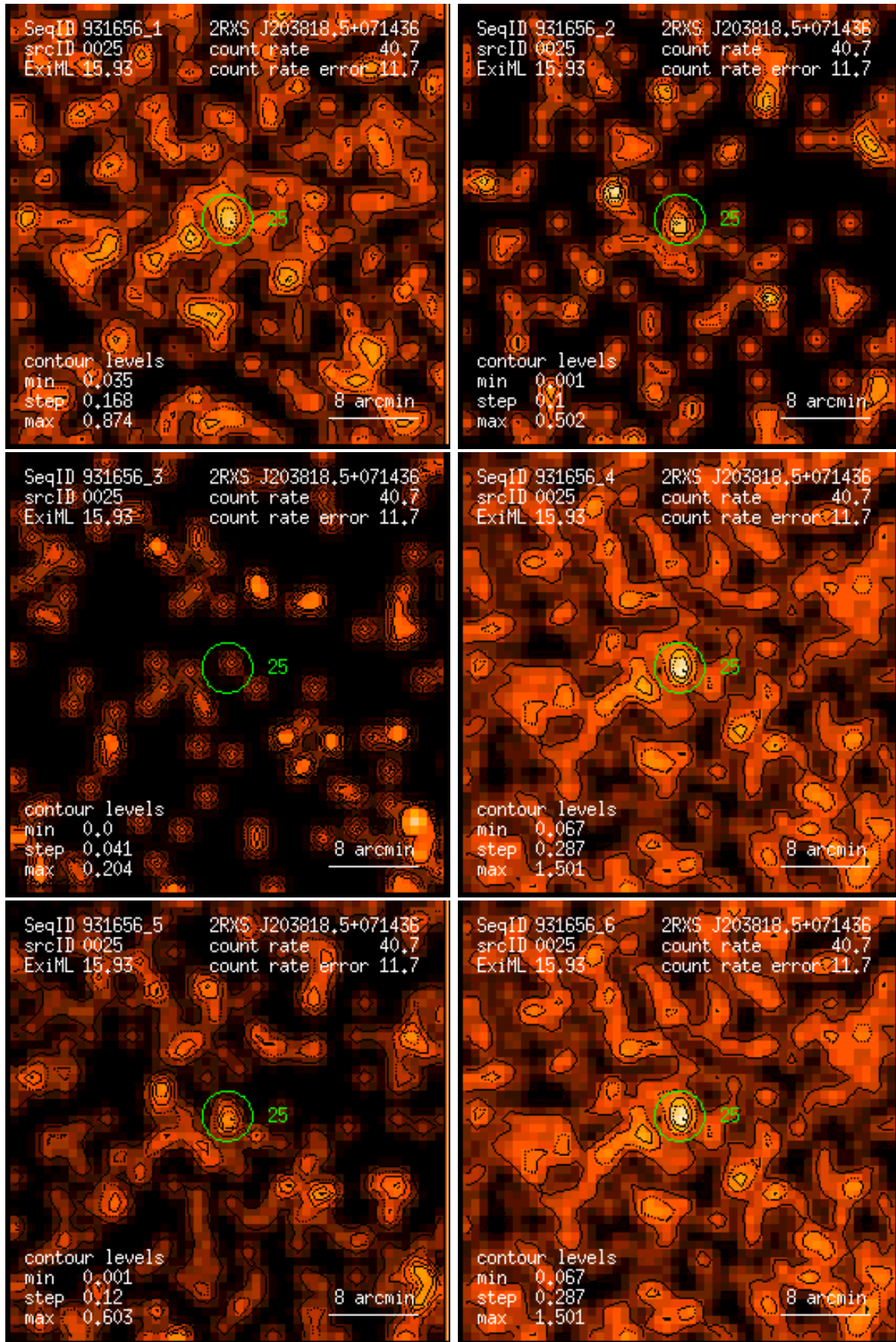
Figure 25: RASS 931656: detection 0025: band rate images, Gaussian filter: (1) PSPC channels 11 – 41, (2) 52 – 90, (3) 91 – 201, (4) 11 – 235, (5) 52 – 201, (6) 11 – 201. Broad band rates in counts/ks. Band rate contour levels in counts/ks/arcmin 2 .
