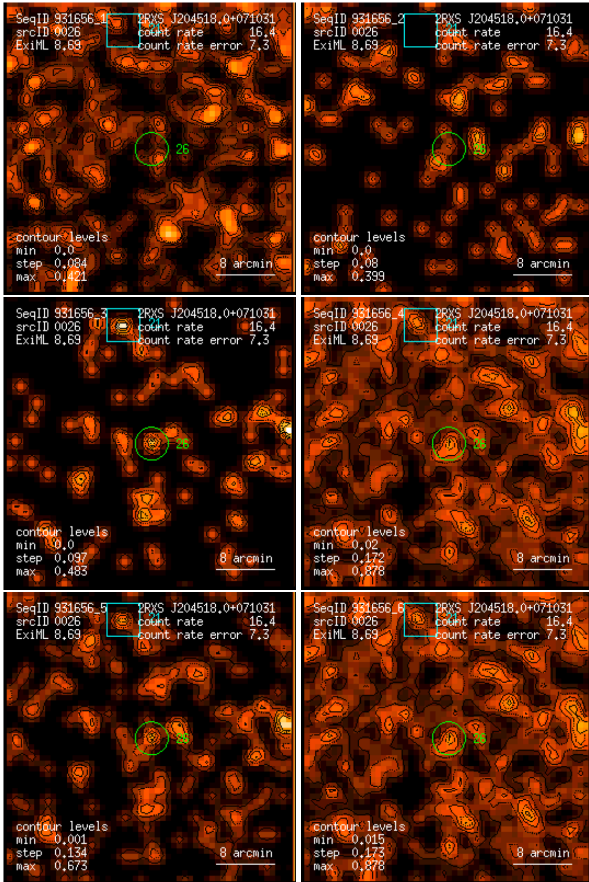
Figure 26: RASS 931656: detection 0026: band rate images, Gaussian filter: (1) PSPC channels 11 – 41, (2) 52 – 90, (3) 91 – 201, (4) 11 – 235, (5) 52 – 201, (6) 11 – 201. Broad band rates in counts/ks. Band rate contour levels in counts/ks/arcmin 2 .
