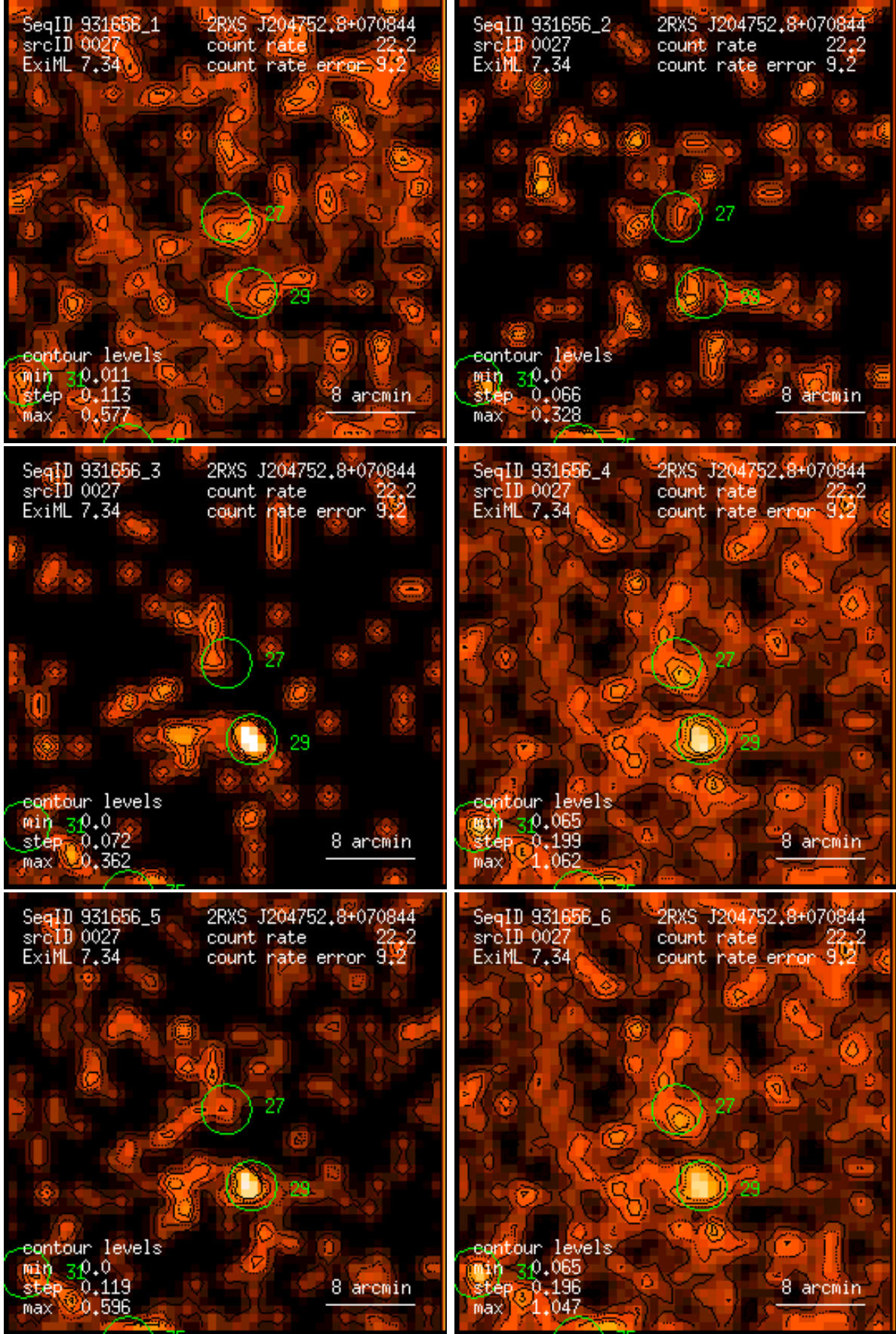
Figure 27: RASS 931656: detection 0027: band rate images, Gaussian filter: (1) PSPC channels 11 – 41, (2) 52 – 90, (3) 91 – 201, (4) 11 – 235, (5) 52 – 201, (6) 11 – 201. Broad band rates in counts/ks. Band rate contour levels in counts/ks/arcmin 2 .
