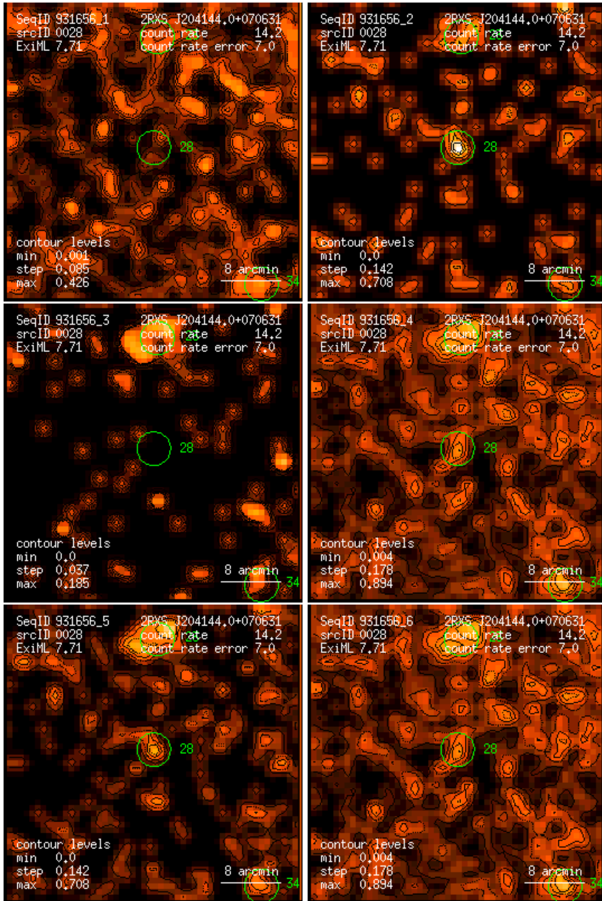
Figure 28: RASS 931656: detection 0028: band rate images, Gaussian filter: (1) PSPC channels 11 – 41, (2) 52 – 90, (3) 91 – 201, (4) 11 – 235, (5) 52 – 201, (6) 11 – 201. Broad band rates in counts/ks. Band rate contour levels in counts/ks/arcmin 2 .
