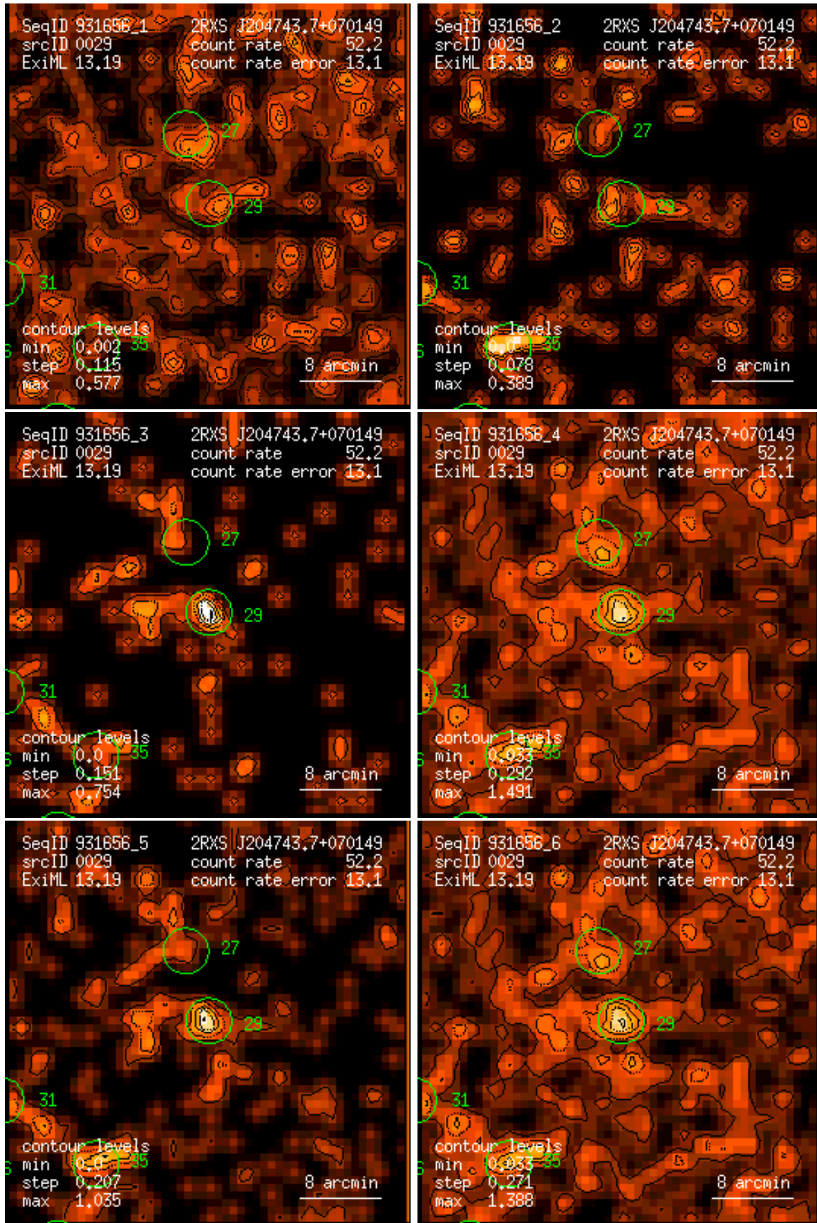
Figure 29: RASS 931656: detection 0029: band rate images, Gaussian filter: (1) PSPC channels 11 – 41, (2) 52 – 90, (3) 91 – 201, (4) 11 – 235, (5) 52 – 201, (6) 11 – 201. Broad band rates in counts/ks. Band rate contour levels in counts/ks/arcmin 2 .
