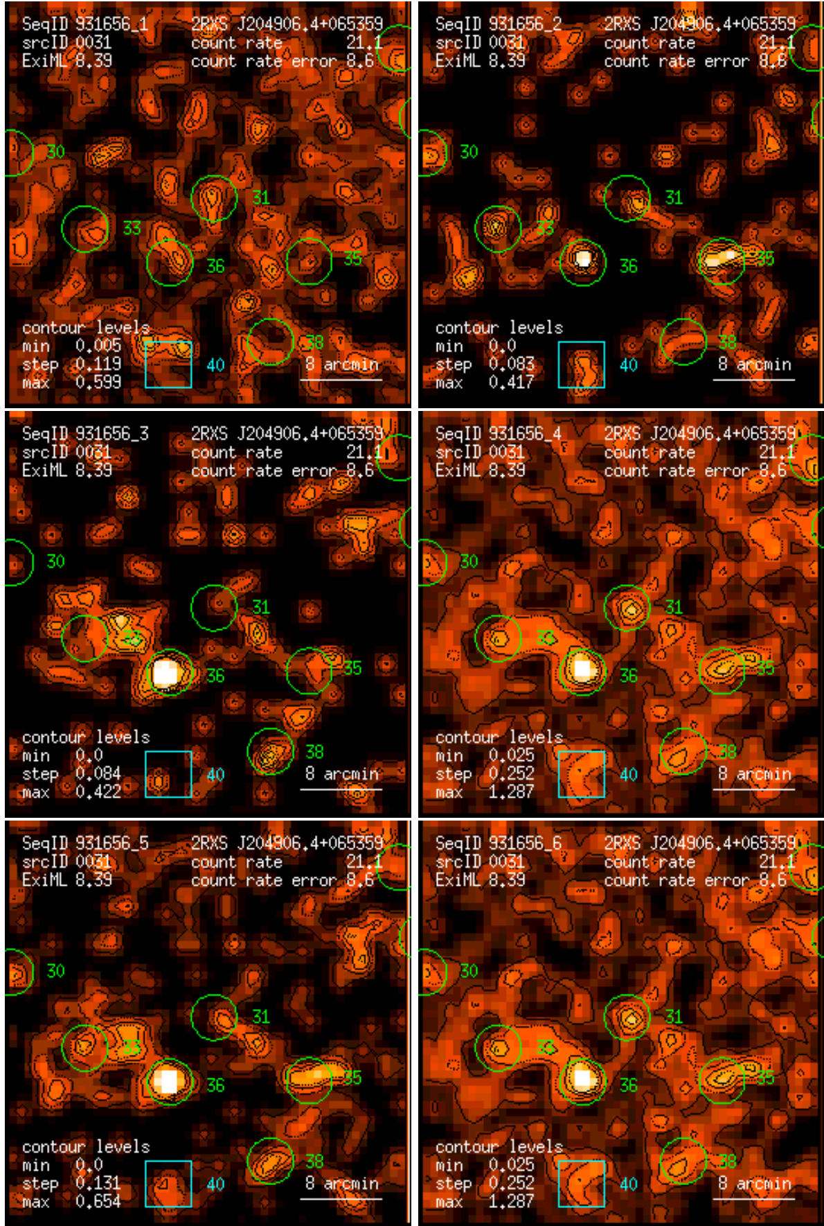
Figure 31: RASS 931656: detection 0031: band rate images, Gaussian filter: (1) PSPC channels 11 – 41, (2) 52 – 90, (3) 91 – 201, (4) 11 – 235, (5) 52 – 201, (6) 11 – 201. Broad band rates in counts/ks. Band rate contour levels in counts/ks/arcmin 2 .
