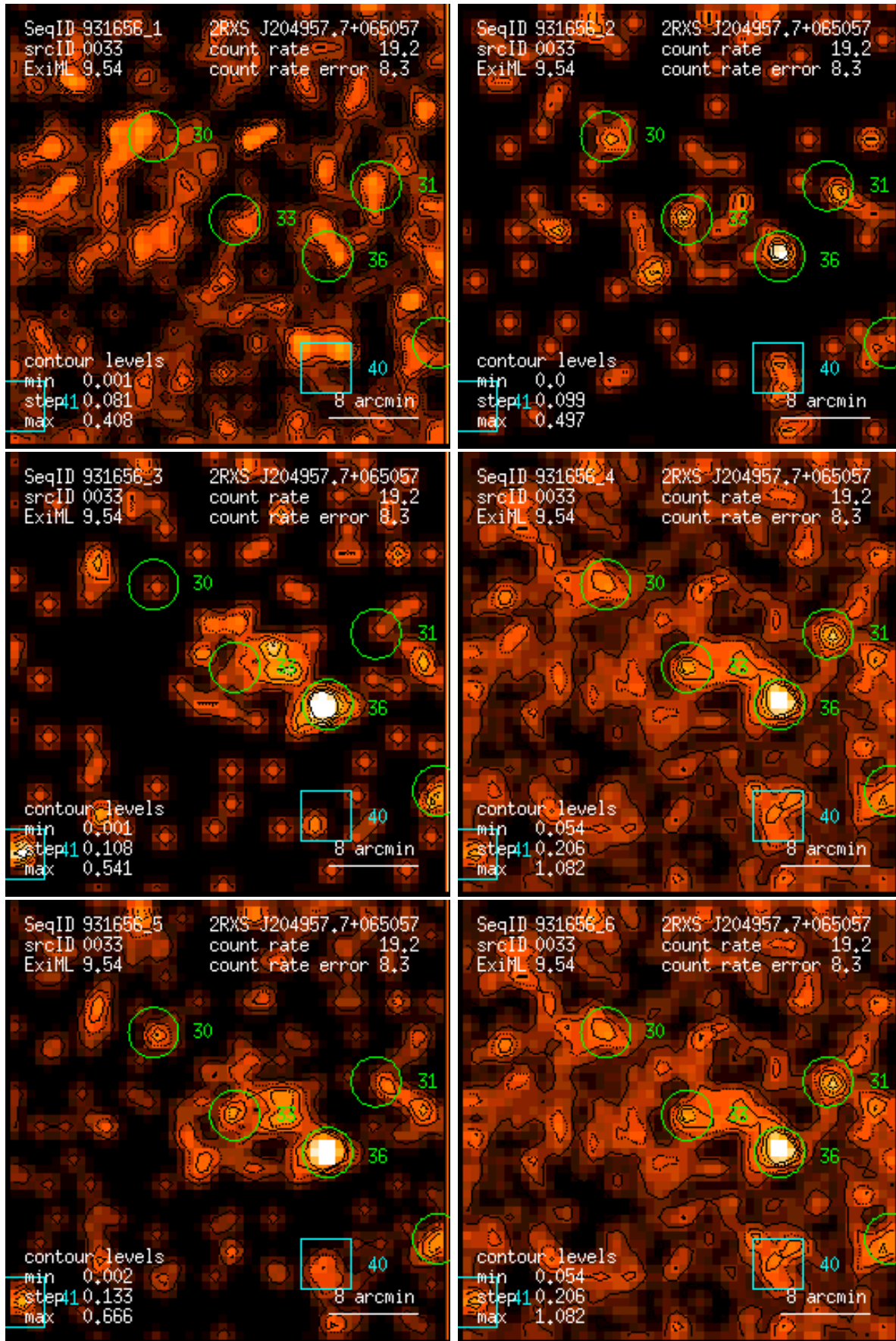
Figure 33: RASS 931656: detection 0033: band rate images, Gaussian filter: (1) PSPC channels 11 – 41, (2) 52 – 90, (3) 91 – 201, (4) 11 – 235, (5) 52 – 201, (6) 11 – 201. Broad band rates in counts/ks. Band rate contour levels in counts/ks/arcmin 2 .
