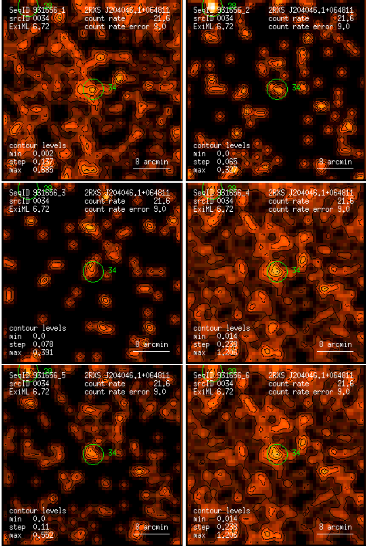
Figure 34: RASS 931656: detection 0034: band rate images, Gaussian filter: (1) PSPC channels 11 – 41, (2) 52 – 90, (3) 91 – 201, (4) 11 – 235, (5) 52 – 201, (6) 11 – 201. Broad band rates in counts/ks. Band rate contour levels in counts/ks/arcmin 2 .
