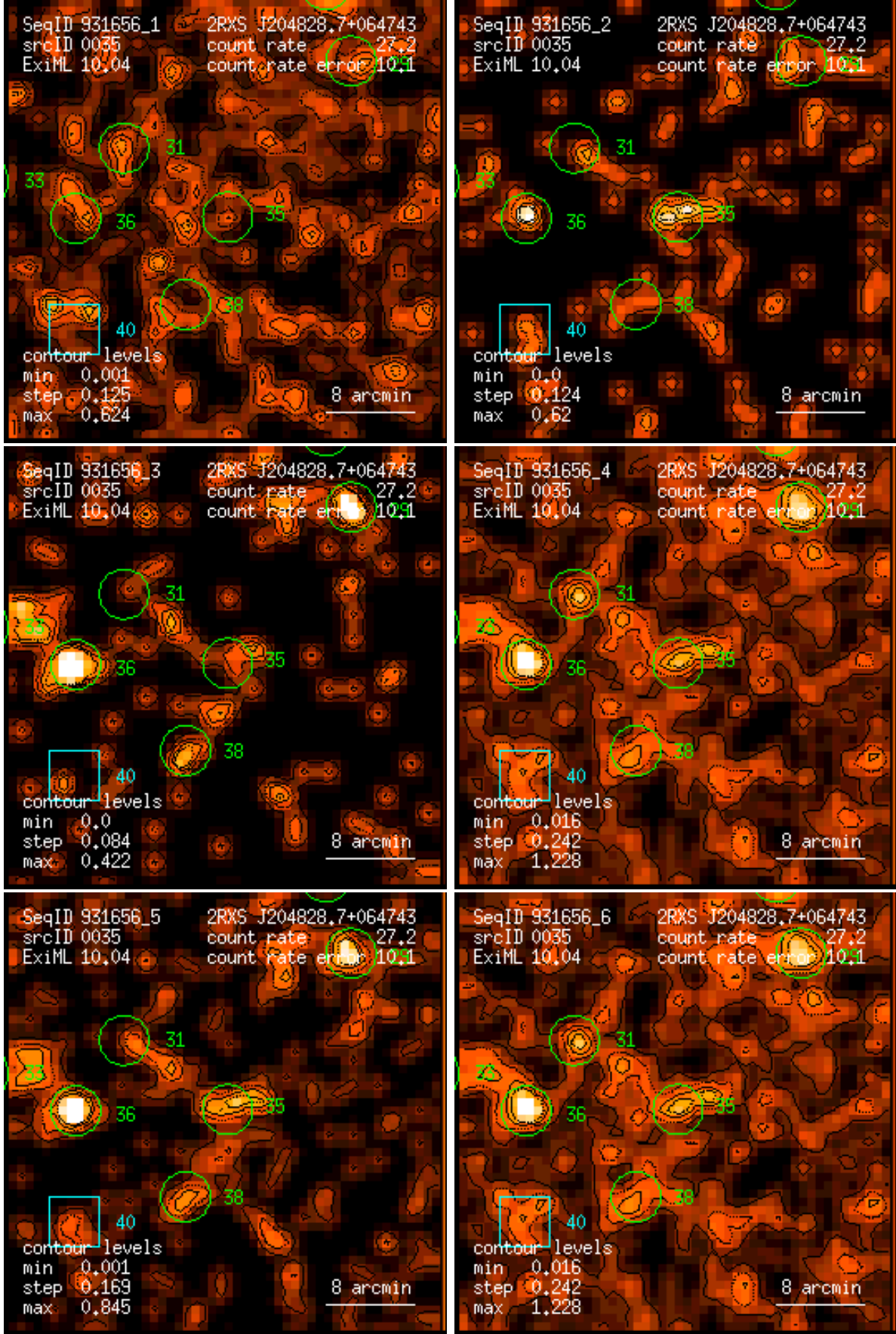
Figure 35: RASS 931656: detection 0035: band rate images, Gaussian filter: (1) PSPC channels 11 – 41, (2) 52 – 90, (3) 91 – 201, (4) 11 – 235, (5) 52 – 201, (6) 11 – 201. Broad band rates in counts/ks. Band rate contour levels in counts/ks/arcmin 2 .
