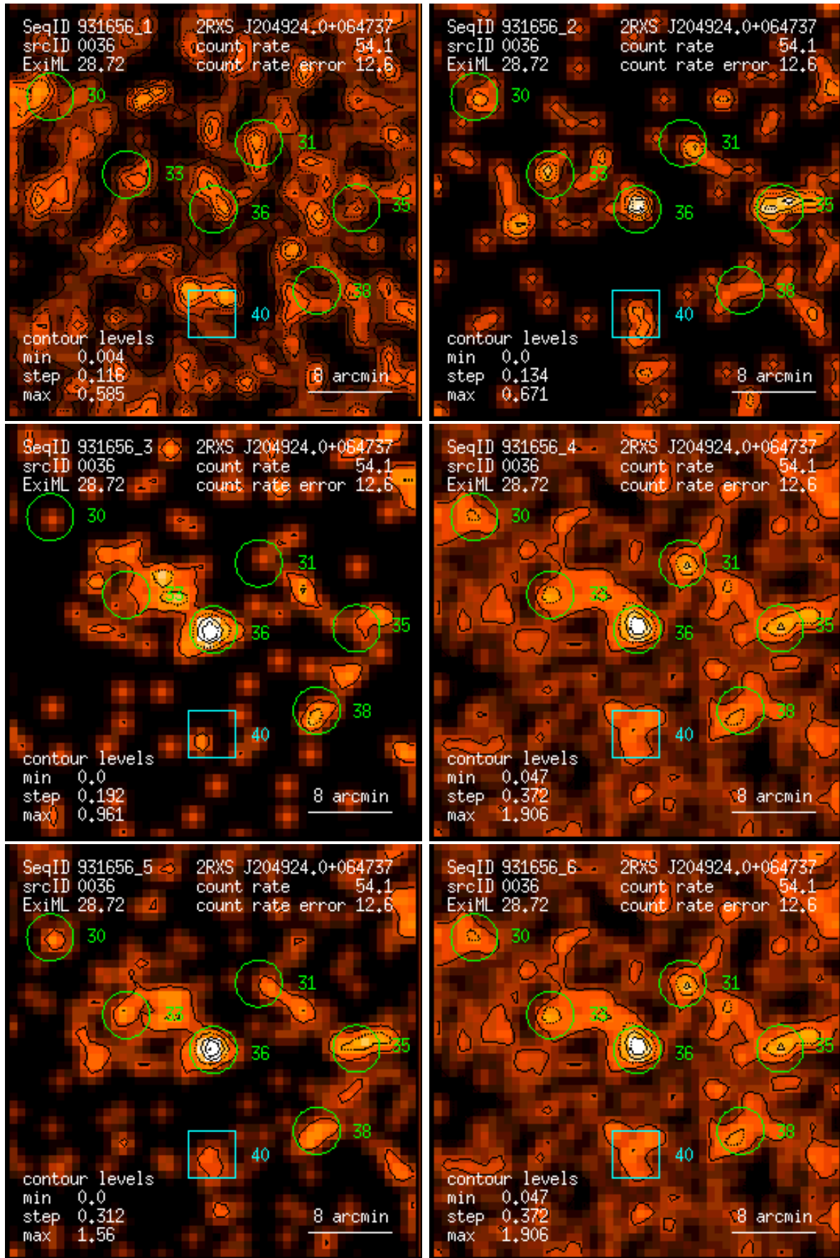
Figure 36: RASS 931656: detection 0036: band rate images, Gaussian filter: (1) PSPC channels 11 – 41, (2) 52 – 90, (3) 91 – 201, (4) 11 – 235, (5) 52 – 201, (6) 11 – 201. Broad band rates in counts/ks. Band rate contour levels in counts/ks/arcmin 2 .
