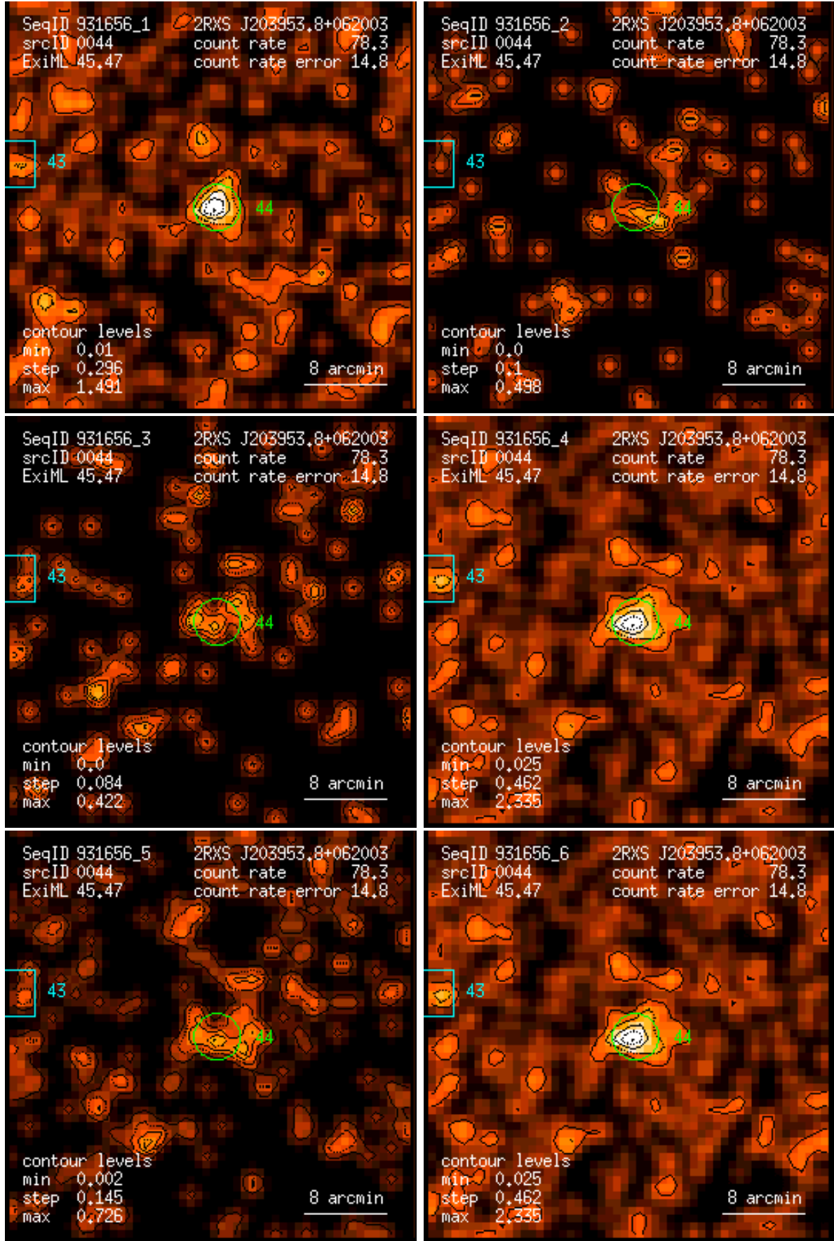
Figure 44: RASS 931656: detection 0044: band rate images, Gaussian filter: (1) PSPC channels 11 – 41, (2) 52 – 90, (3) 91 – 201, (4) 11 – 235, (5) 52 – 201, (6) 11 – 201. Broad band rates in counts/ks. Band rate contour levels in counts/ks/arcmin 2 .
