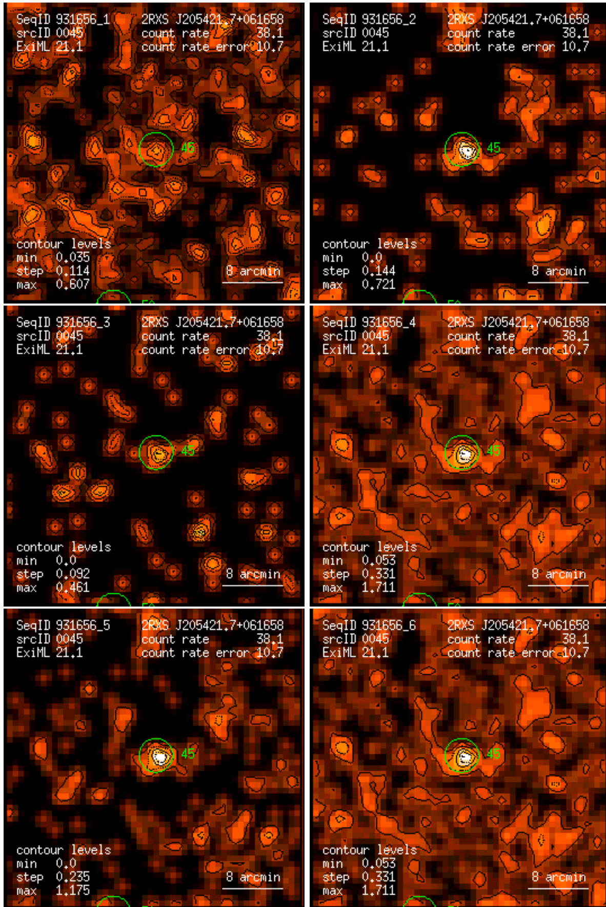
Figure 45: RASS 931656: detection 0045: band rate images, Gaussian filter: (1) PSPC channels 11 – 41, (2) 52 – 90, (3) 91 – 201, (4) 11 – 235, (5) 52 – 201, (6) 11 – 201. Broad band rates in counts/ks. Band rate contour levels in counts/ks/arcmin 2 .
