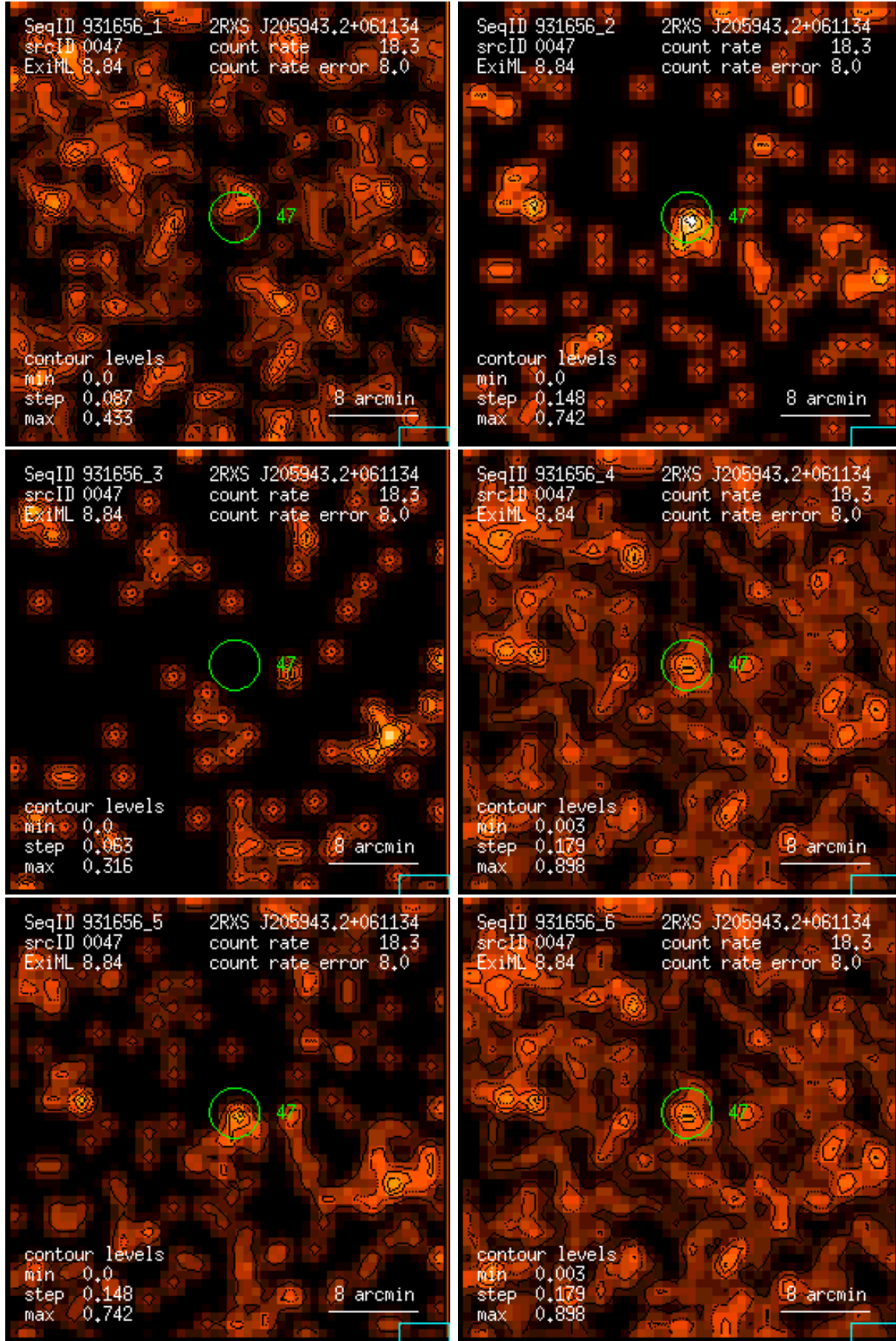
Figure 47: RASS 931656: detection 0047: band rate images, Gaussian filter: (1) PSPC channels 11 – 41, (2) 52 – 90, (3) 91 – 201, (4) 11 – 235, (5) 52 – 201, (6) 11 – 201. Broad band rates in counts/ks. Band rate contour levels in counts/ks/arcmin 2 .
