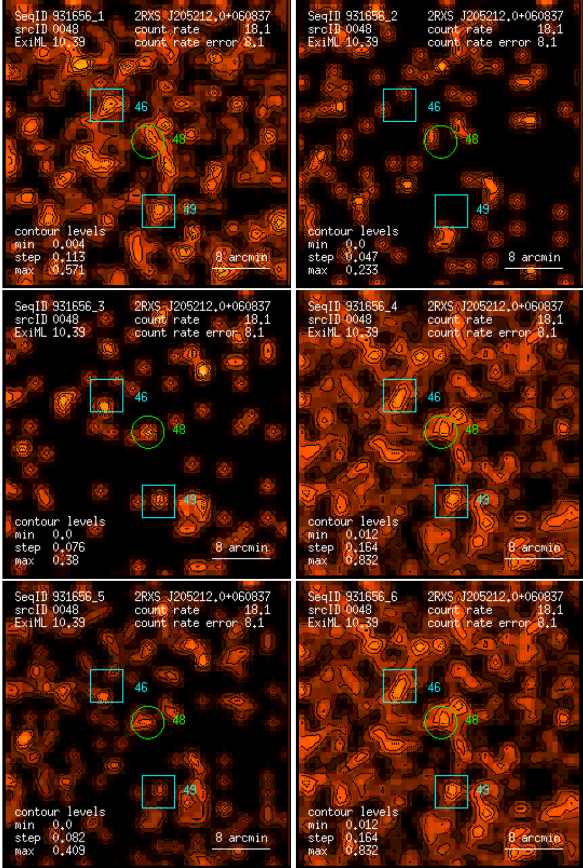
Figure 48: RASS 931656: detection 0048: band rate images, Gaussian filter: (1) PSPC channels 11 – 41, (2) 52 – 90, (3) 91 – 201, (4) 11 – 235, (5) 52 – 201, (6) 11 – 201. Broad band rates in counts/ks. Band rate contour levels in counts/ks/arcmin 2 .
