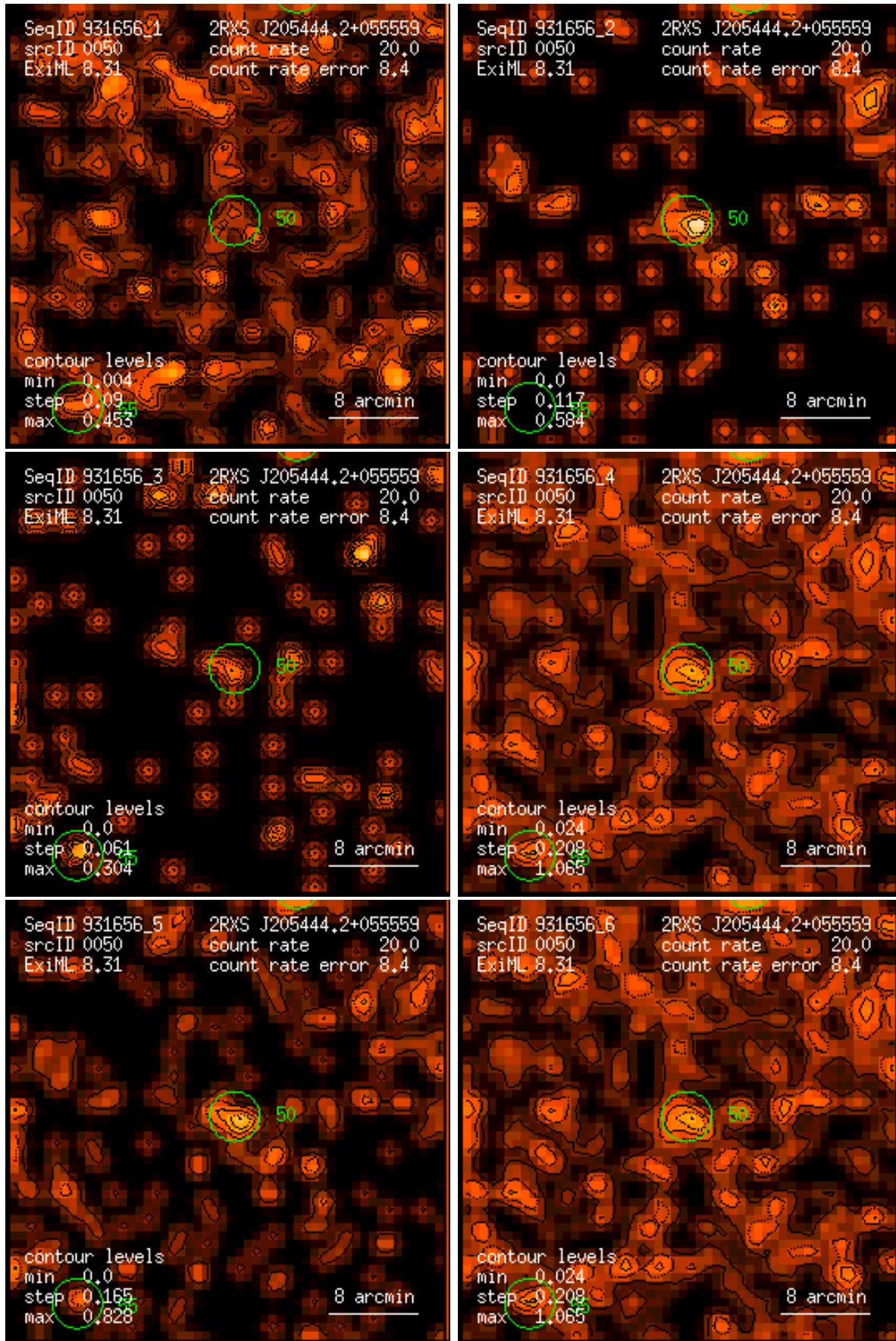
Figure 50: RASS 931656: detection 0050: band rate images, Gaussian filter: (1) PSPC channels 11 – 41, (2) 52 – 90, (3) 91 – 201, (4) 11 – 235, (5) 52 – 201, (6) 11 – 201. Broad band rates in counts/ks. Band rate contour levels in counts/ks/arcmin 2 .
