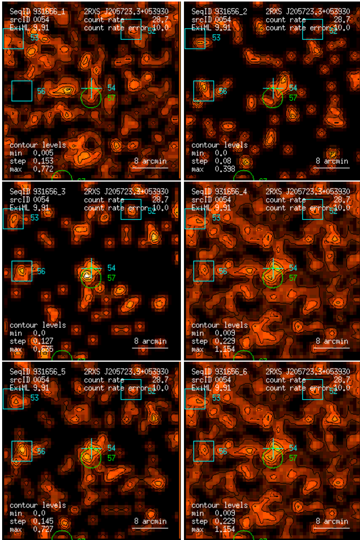
Figure 54: RASS 931656: detection 0054: band rate images, Gaussian filter: (1) PSPC channels 11 – 41, (2) 52 – 90, (3) 91 – 201, (4) 11 – 235, (5) 52 – 201, (6) 11 – 201. Broad band rates in counts/ks. Band rate contour levels in counts/ks/arcmin 2 .
