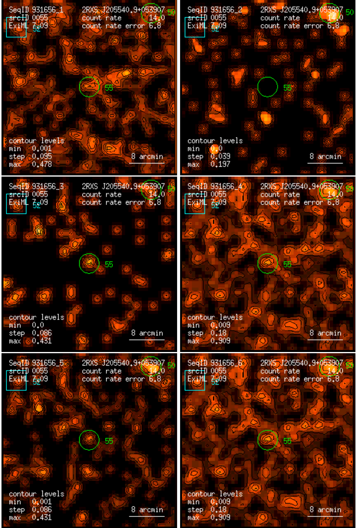
Figure 55: RASS 931656: detection 0055: band rate images, Gaussian filter: (1) PSPC channels 11 – 41, (2) 52 – 90, (3) 91 – 201, (4) 11 – 235, (5) 52 – 201, (6) 11 – 201. Broad band rates in counts/ks. Band rate contour levels in counts/ks/arcmin 2 .
