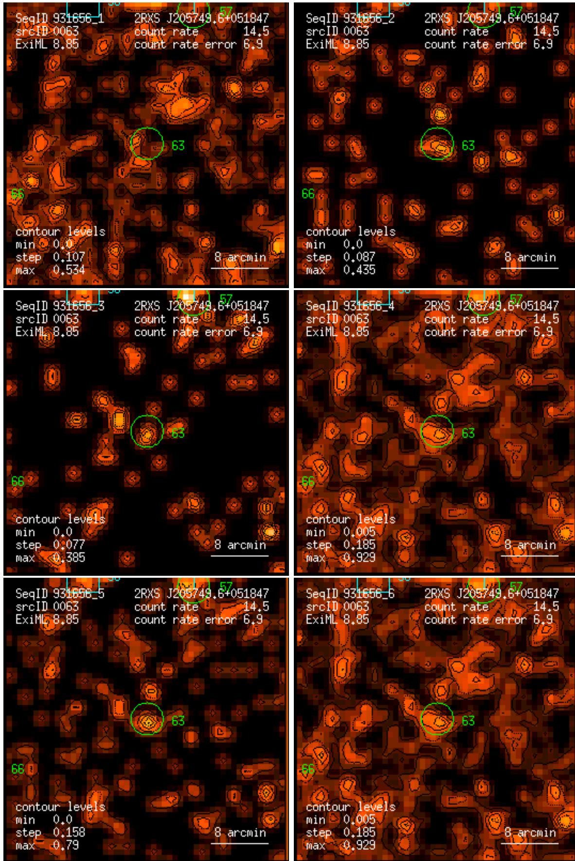
Figure 63: RASS 931656: detection 0063: band rate images, Gaussian filter: (1) PSPC channels 11 – 41, (2) 52 – 90, (3) 91 – 201, (4) 11 – 235, (5) 52 – 201, (6) 11 – 201. Broad band rates in counts/ks. Band rate contour levels in counts/ks/arcmin 2 .
