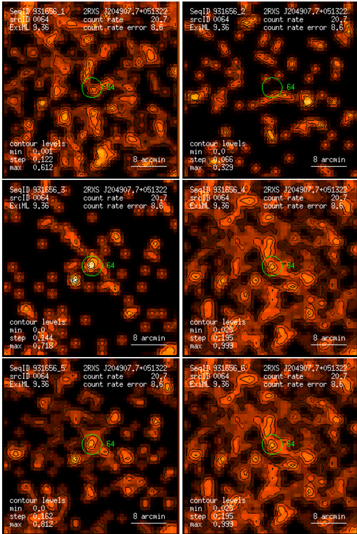
Figure 64: RASS 931656: detection 0064: band rate images, Gaussian filter: (1) PSPC channels 11 – 41, (2) 52 – 90, (3) 91 – 201, (4) 11 – 235, (5) 52 – 201, (6) 11 – 201. Broad band rates in counts/ks. Band rate contour levels in counts/ks/arcmin 2 .
