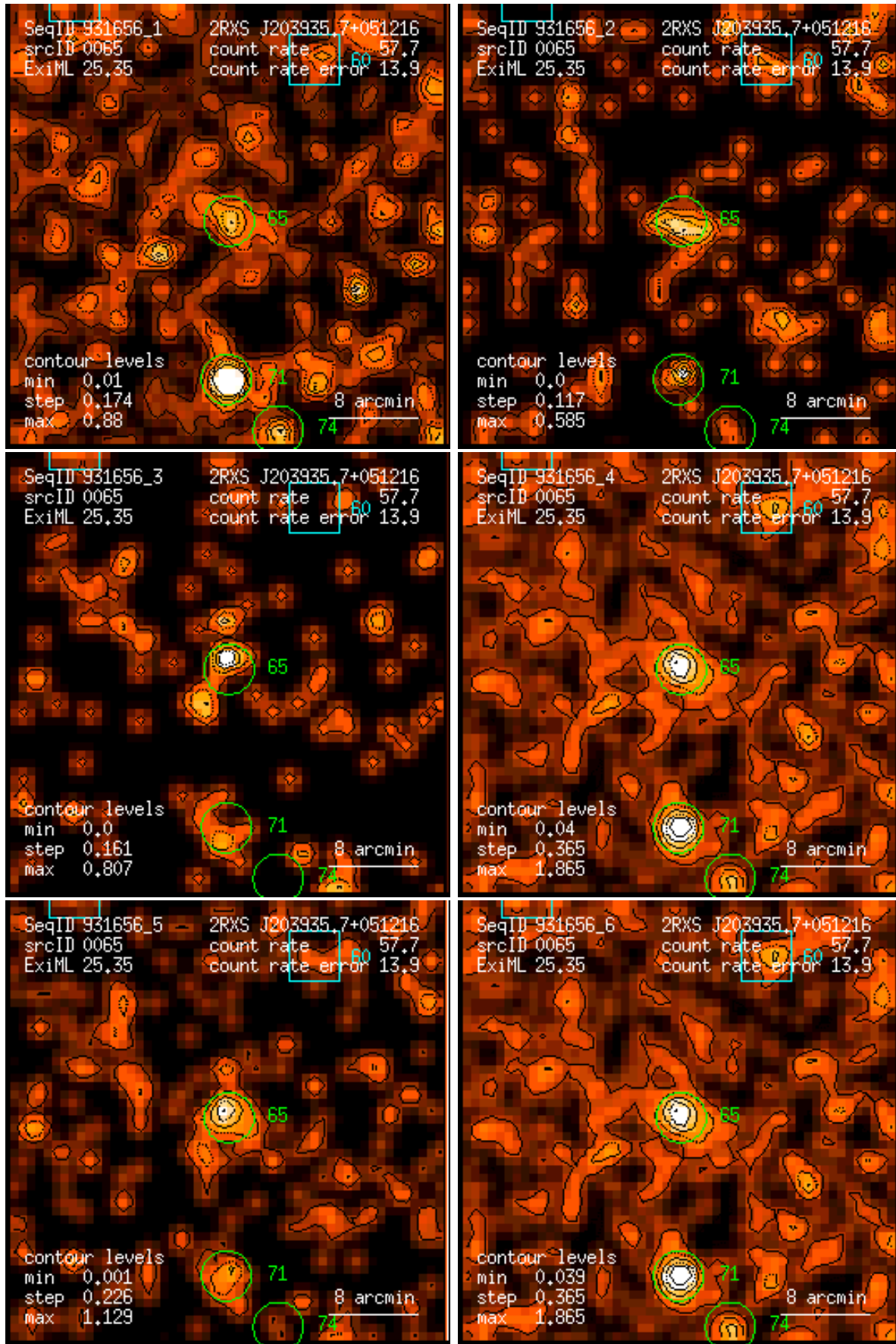
Figure 65: RASS 931656: detection 0065: band rate images, Gaussian filter: (1) PSPC channels 11 – 41, (2) 52 – 90, (3) 91 – 201, (4) 11 – 235, (5) 52 – 201, (6) 11 – 201. Broad band rates in counts/ks. Band rate contour levels in counts/ks/arcmin 2 .
