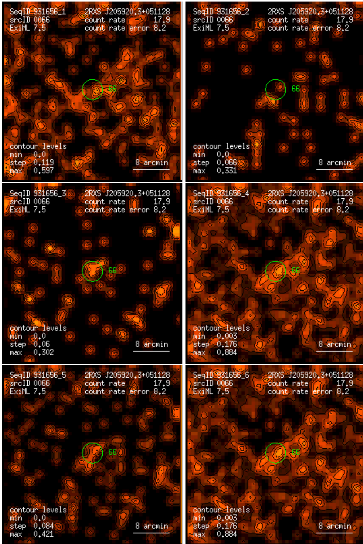
Figure 66: RASS 931656: detection 0066: band rate images, Gaussian filter: (1) PSPC channels 11 – 41, (2) 52 – 90, (3) 91 – 201, (4) 11 – 235, (5) 52 – 201, (6) 11 – 201. Broad band rates in counts/ks. Band rate contour levels in counts/ks/arcmin 2 .
