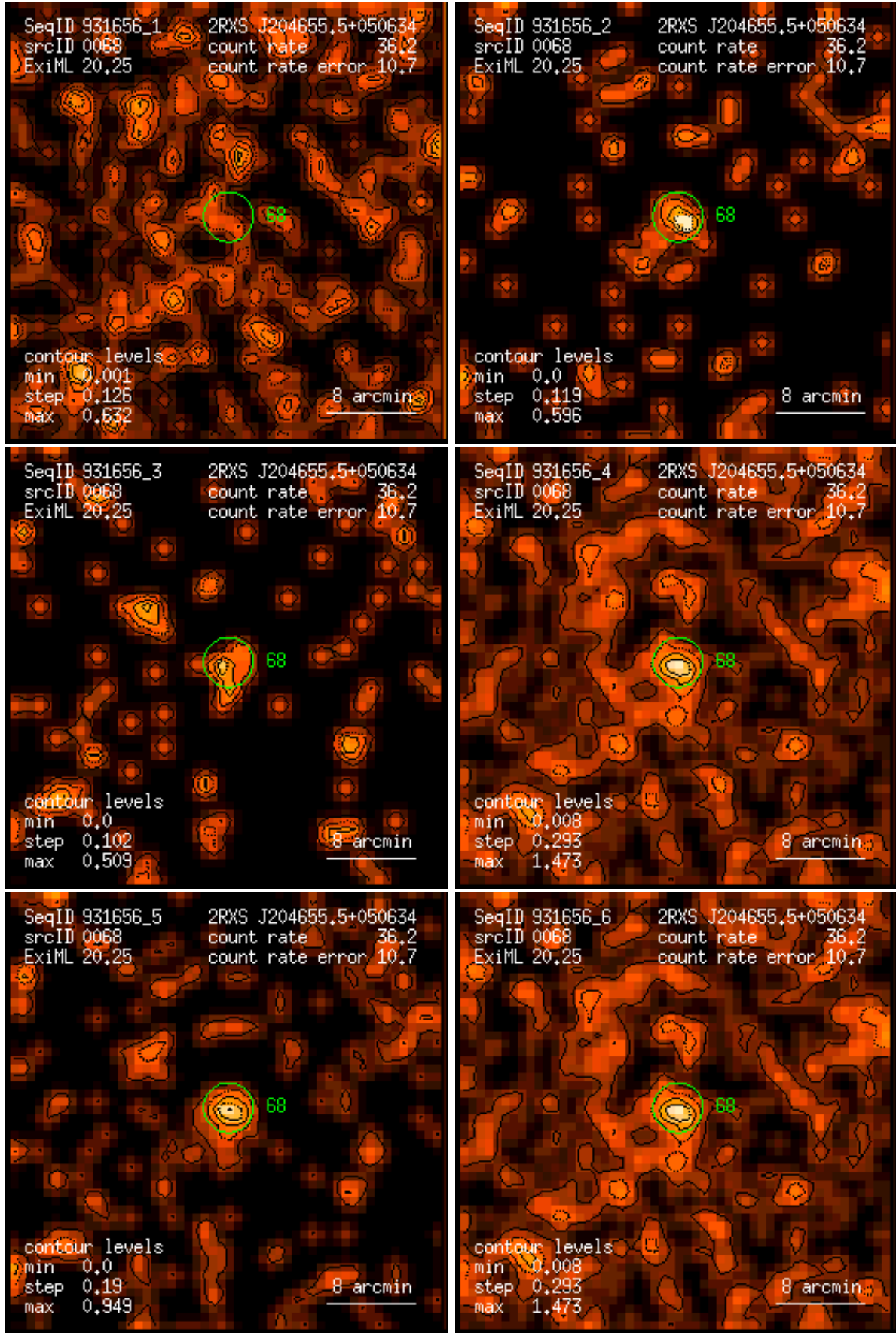
Figure 68: RASS 931656: detection 0068: band rate images, Gaussian filter: (1) PSPC channels 11 – 41, (2) 52 – 90, (3) 91 – 201, (4) 11 – 235, (5) 52 – 201, (6) 11 – 201. Broad band rates in counts/ks. Band rate contour levels in counts/ks/arcmin 2 .
