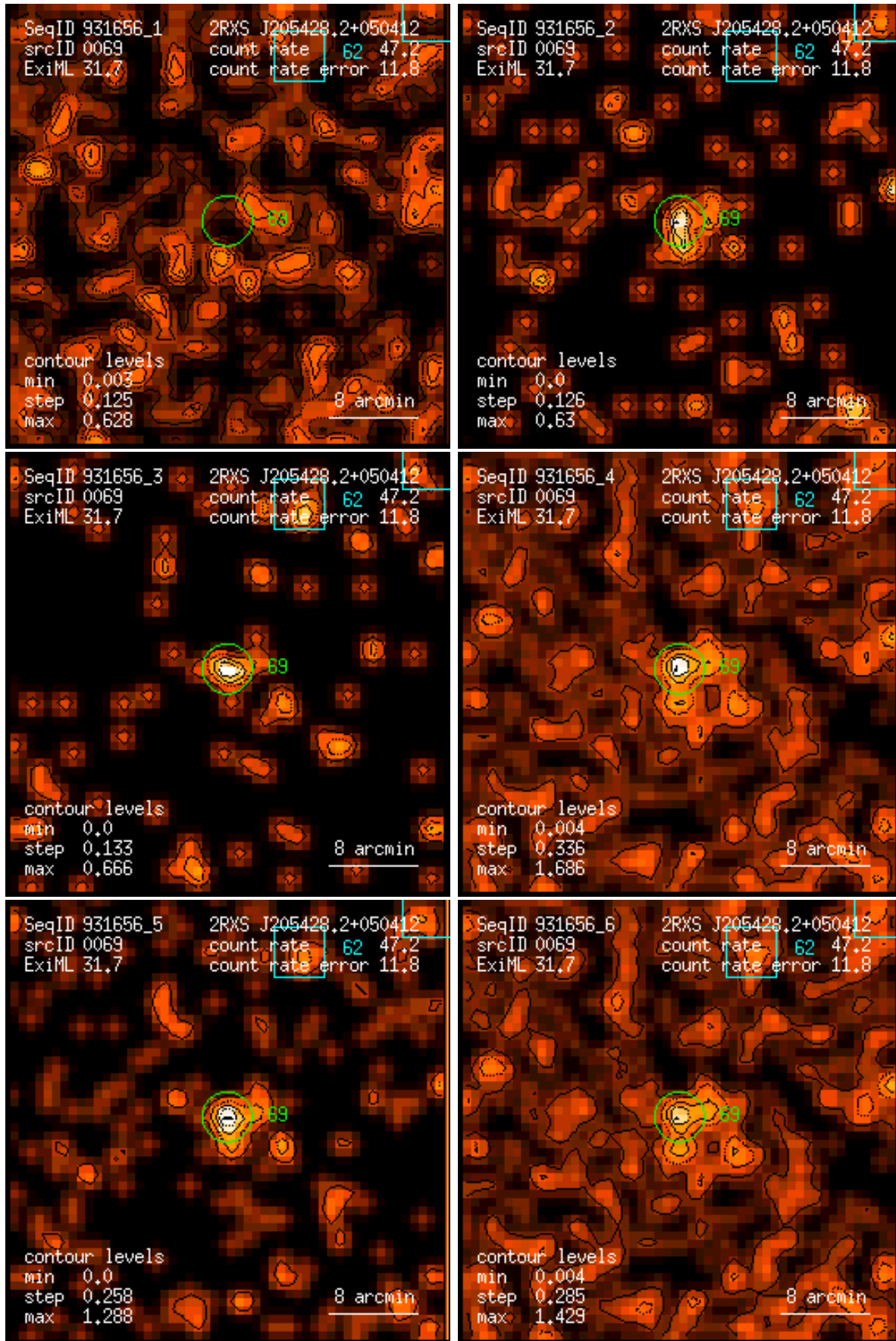
Figure 69: RASS 931656: detection 0069: band rate images, Gaussian filter: (1) PSPC channels 11 – 41, (2) 52 – 90, (3) 91 – 201, (4) 11 – 235, (5) 52 – 201, (6) 11 – 201. Broad band rates in counts/ks. Band rate contour levels in counts/ks/arcmin 2 .
