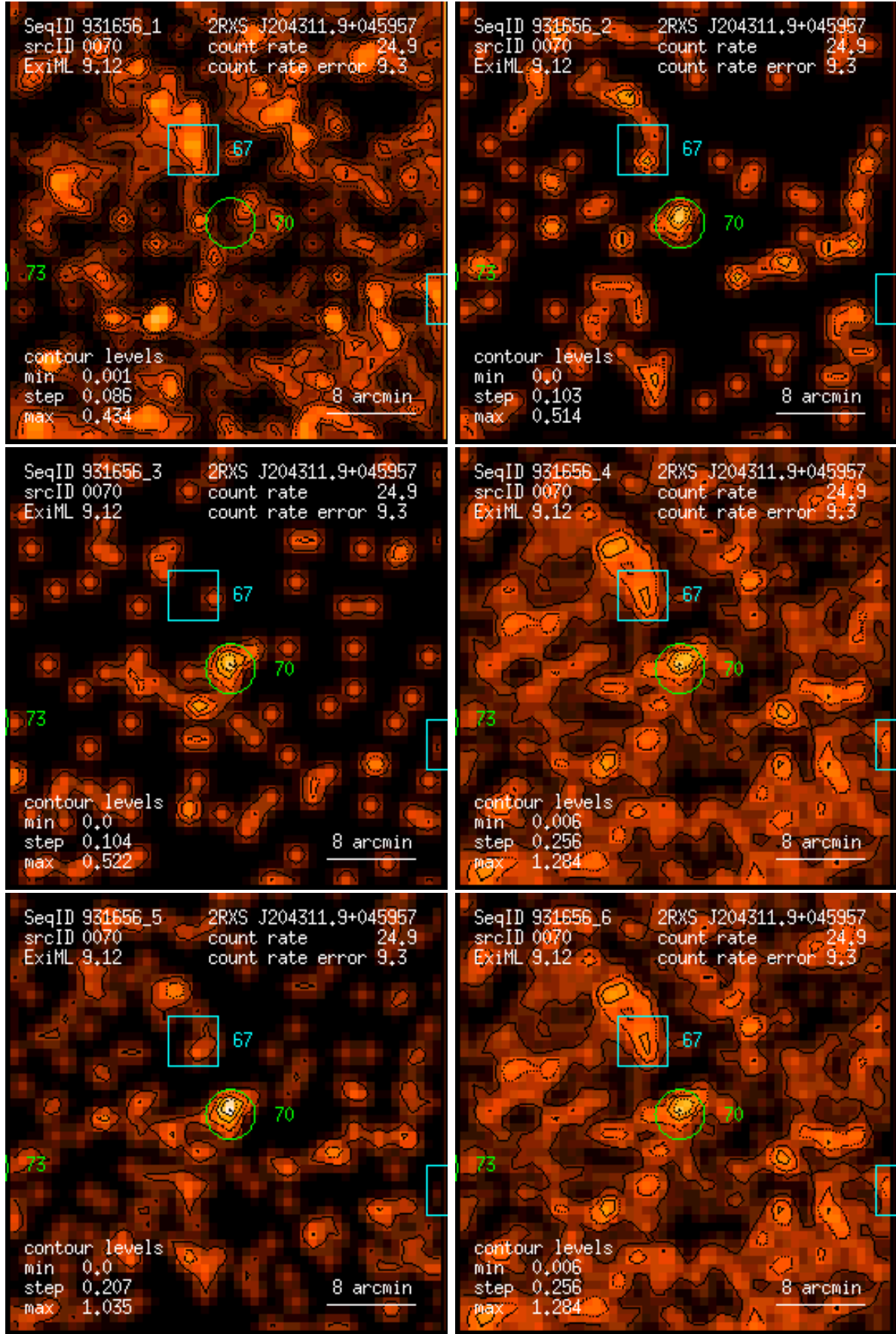
Figure 70: RASS 931656: detection 0070: band rate images, Gaussian filter: (1) PSPC channels 11 – 41, (2) 52 – 90, (3) 91 – 201, (4) 11 – 235, (5) 52 – 201, (6) 11 – 201. Broad band rates in counts/ks. Band rate contour levels in counts/ks/arcmin 2 .
