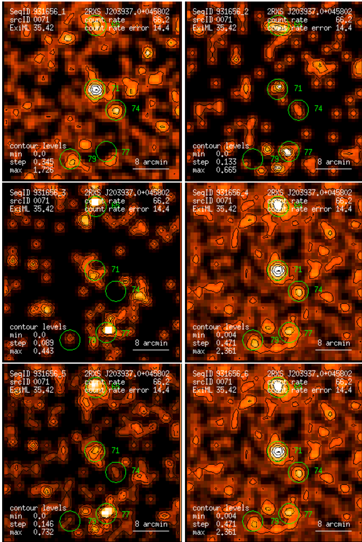
Figure 71: RASS 931656: detection 0071: band rate images, Gaussian filter: (1) PSPC channels 11 – 41, (2) 52 – 90, (3) 91 – 201, (4) 11 – 235, (5) 52 – 201, (6) 11 – 201. Broad band rates in counts/ks. Band rate contour levels in counts/ks/arcmin 2 .
