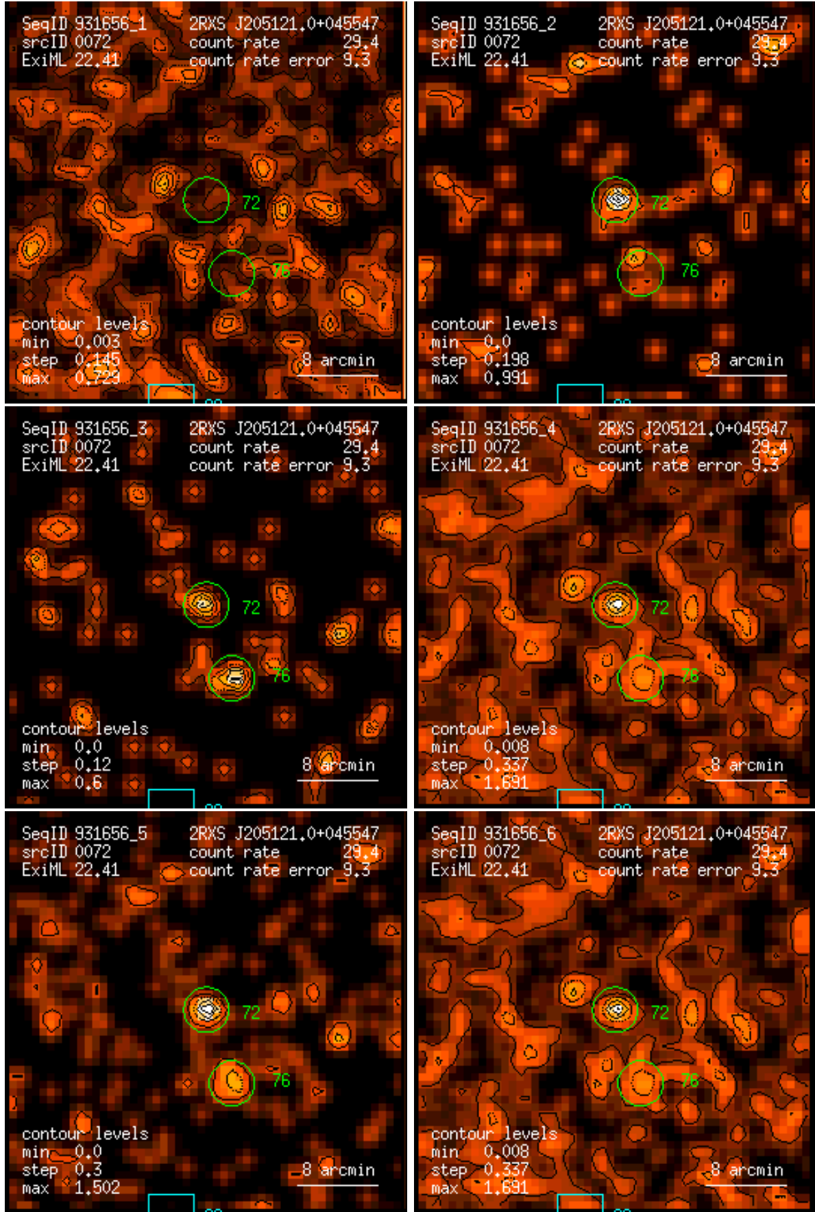
Figure 72: RASS 931656: detection 0072: band rate images, Gaussian filter: (1) PSPC channels 11 – 41, (2) 52 – 90, (3) 91 – 201, (4) 11 – 235, (5) 52 – 201, (6) 11 – 201. Broad band rates in counts/ks. Band rate contour levels in counts/ks/arcmin 2 .
