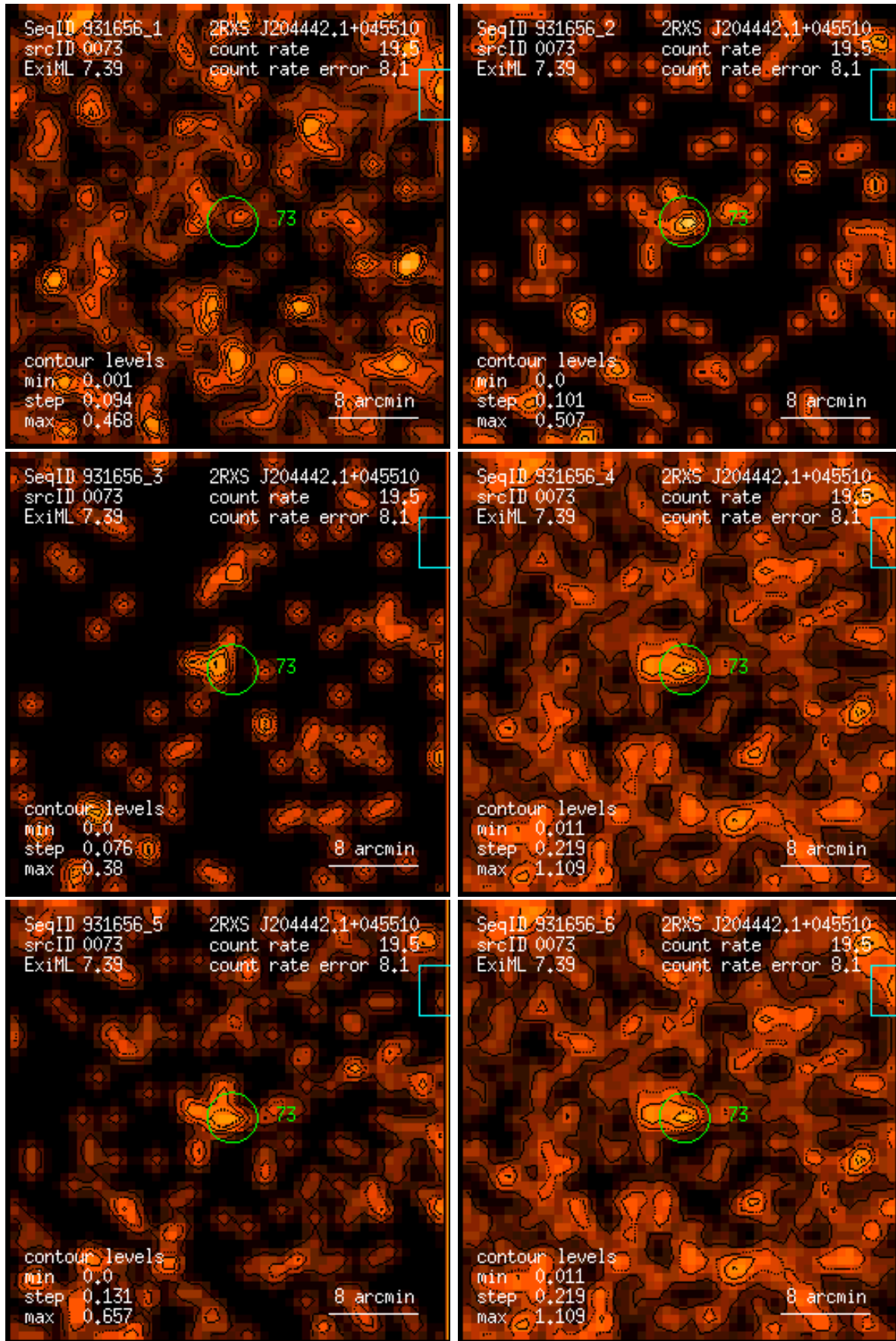
Figure 73: RASS 931656: detection 0073: band rate images, Gaussian filter: (1) PSPC channels 11 – 41, (2) 52 – 90, (3) 91 – 201, (4) 11 – 235, (5) 52 – 201, (6) 11 – 201. Broad band rates in counts/ks. Band rate contour levels in counts/ks/arcmin 2 .
