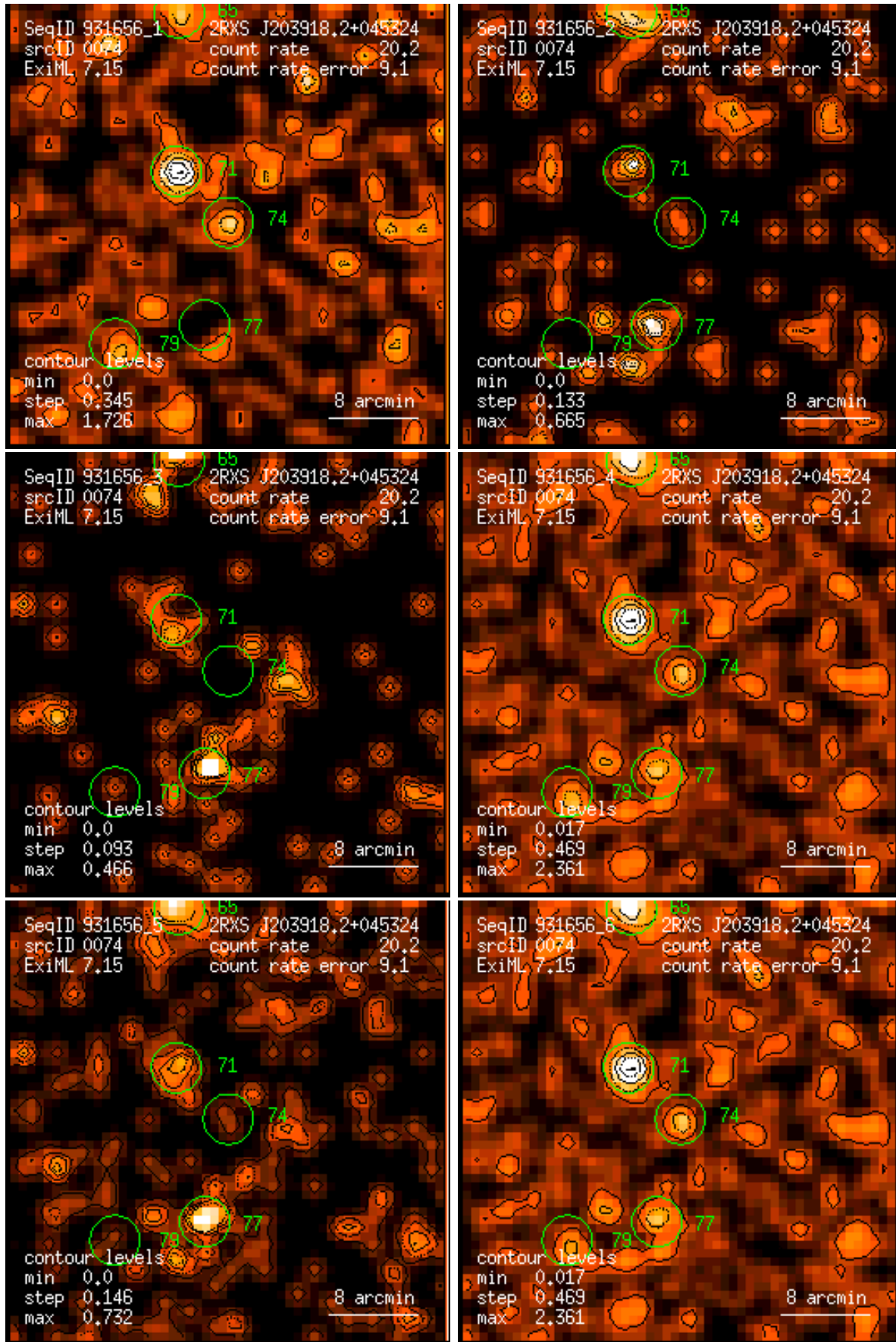
Figure 74: RASS 931656: detection 0074: band rate images, Gaussian filter: (1) PSPC channels 11 – 41, (2) 52 – 90, (3) 91 – 201, (4) 11 – 235, (5) 52 – 201, (6) 11 – 201. Broad band rates in counts/ks. Band rate contour levels in counts/ks/arcmin 2 .
