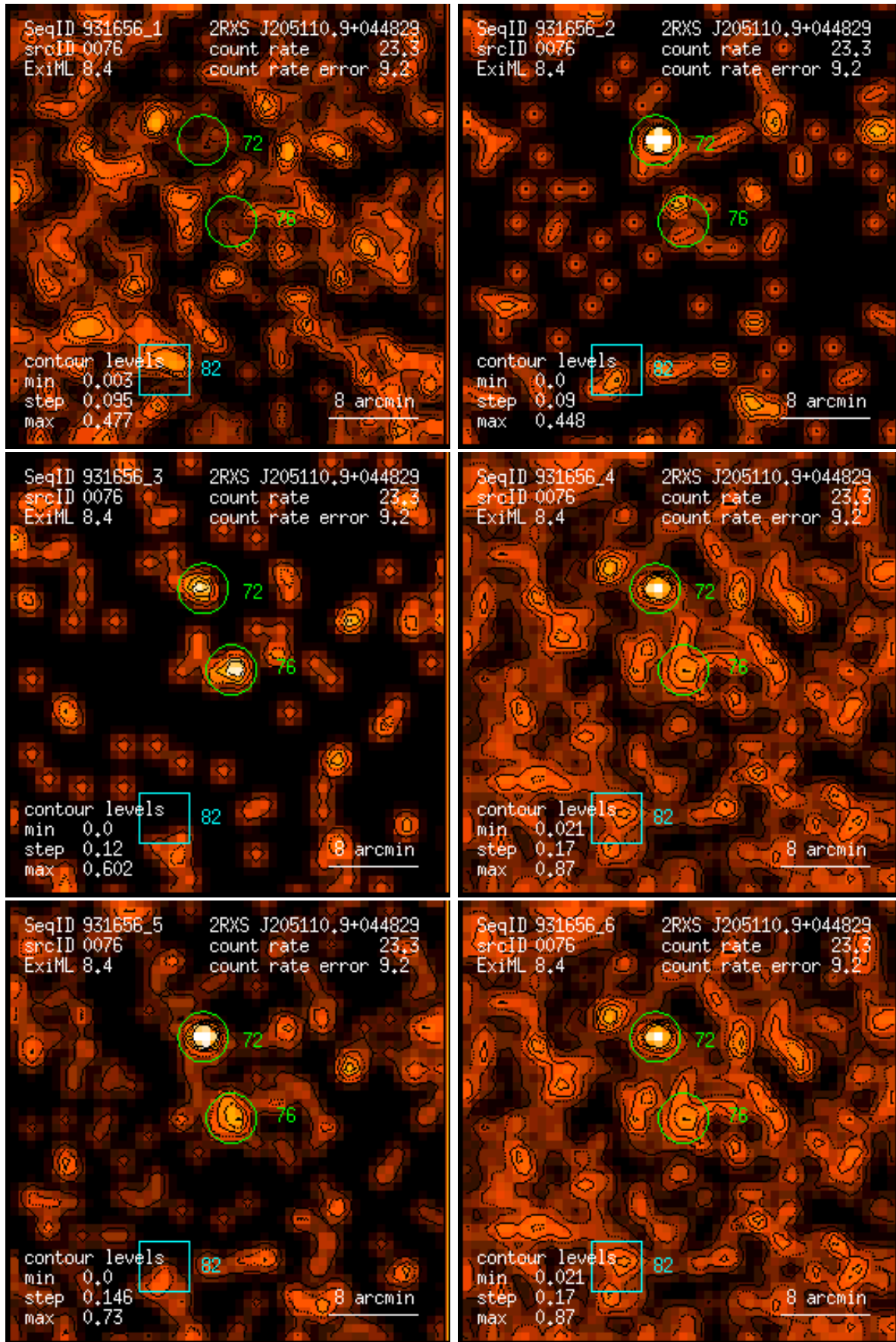
Figure 76: RASS 931656: detection 0076: band rate images, Gaussian filter: (1) PSPC channels 11 – 41, (2) 52 – 90, (3) 91 – 201, (4) 11 – 235, (5) 52 – 201, (6) 11 – 201. Broad band rates in counts/ks. Band rate contour levels in counts/ks/arcmin 2 .
