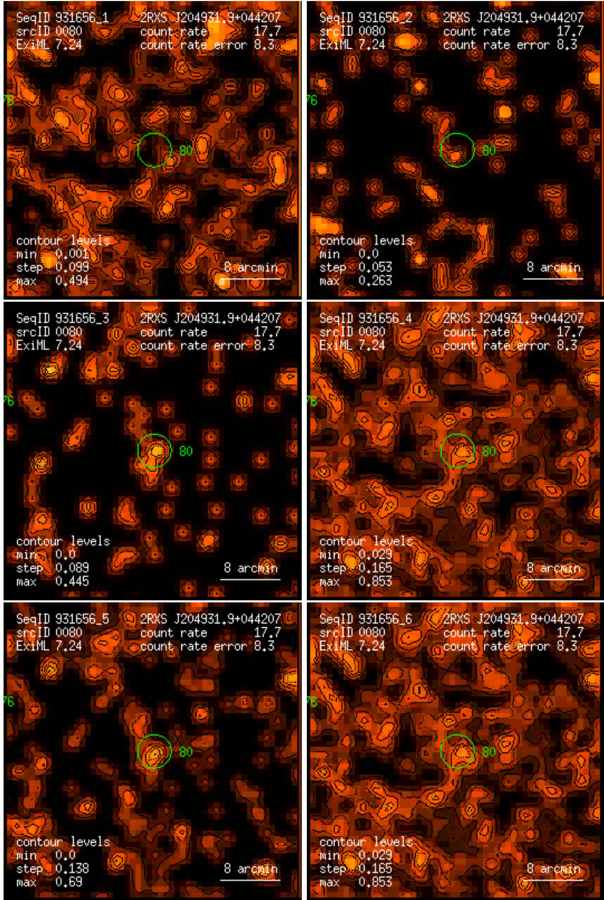
Figure 80: RASS 931656: detection 0080: band rate images, Gaussian filter: (1) PSPC channels 11 – 41, (2) 52 – 90, (3) 91 – 201, (4) 11 – 235, (5) 52 – 201, (6) 11 – 201. Broad band rates in counts/ks. Band rate contour levels in counts/ks/arcmin 2 .
