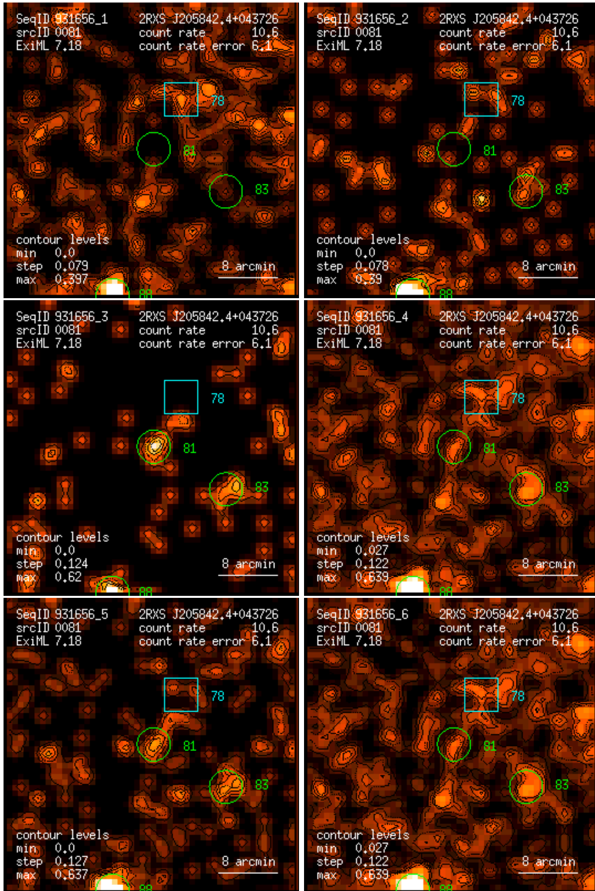
Figure 81: RASS 931656: detection 0081: band rate images, Gaussian filter: (1) PSPC channels 11 – 41, (2) 52 – 90, (3) 91 – 201, (4) 11 – 235, (5) 52 – 201, (6) 11 – 201. Broad band rates in counts/ks. Band rate contour levels in counts/ks/arcmin 2 .
