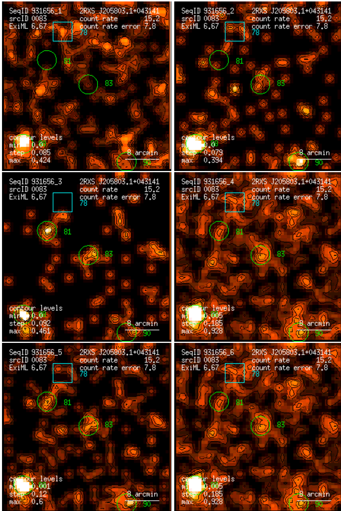
Figure 83: RASS 931656: detection 0083: band rate images, Gaussian filter: (1) PSPC channels 11 – 41, (2) 52 – 90, (3) 91 – 201, (4) 11 – 235, (5) 52 – 201, (6) 11 – 201. Broad band rates in counts/ks. Band rate contour levels in counts/ks/arcmin 2 .
