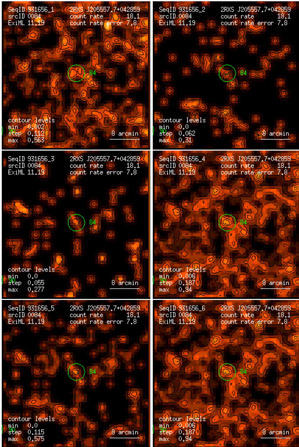
Figure 84: RASS 931656: detection 0084: band rate images, Gaussian filter: (1) PSPC channels 11 – 41, (2) 52 – 90, (3) 91 – 201, (4) 11 – 235, (5) 52 – 201, (6) 11 – 201. Broad band rates in counts/ks. Band rate contour levels in counts/ks/arcmin 2 .
