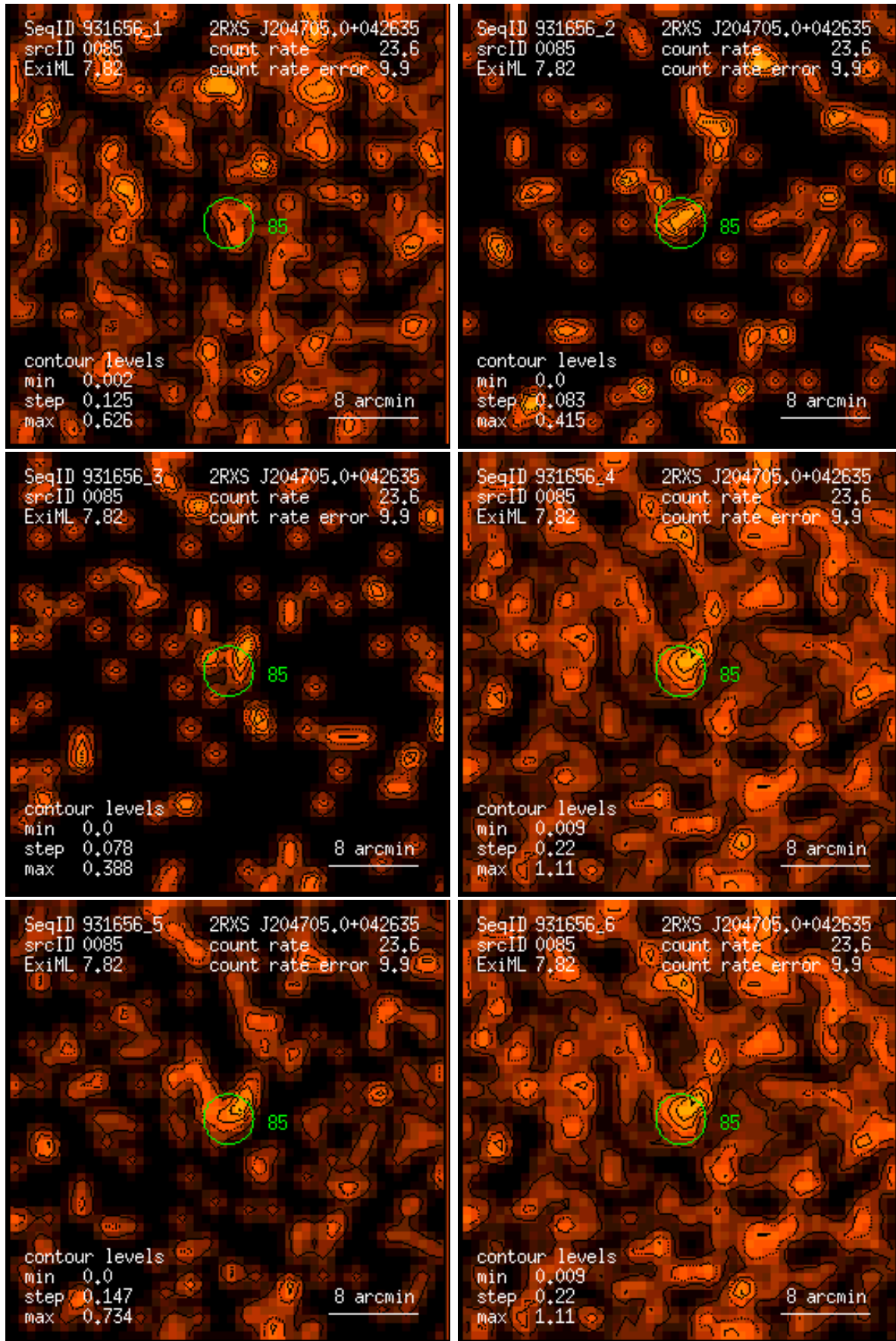
Figure 85: RASS 931656: detection 0085: band rate images, Gaussian filter: (1) PSPC channels 11 – 41, (2) 52 – 90, (3) 91 – 201, (4) 11 – 235, (5) 52 – 201, (6) 11 – 201. Broad band rates in counts/ks. Band rate contour levels in counts/ks/arcmin 2 .
