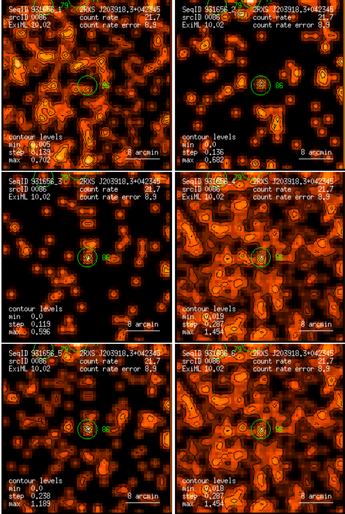
Figure 86: RASS 931656: detection 0086: band rate images, Gaussian filter: (1) PSPC channels 11 – 41, (2) 52 – 90, (3) 91 – 201, (4) 11 – 235, (5) 52 – 201, (6) 11 – 201. Broad band rates in counts/ks. Band rate contour levels in counts/ks/arcmin 2 .
